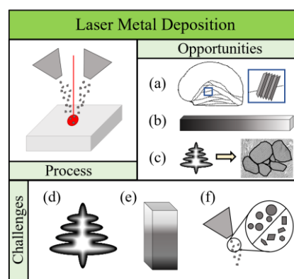
Figure 1: LMD has distinct opportunities and challenges including (a) grains grow epitaxially from substrate over multiple print layers, (b) gradient properties are possible, (c) heat treatment homogenizes samples; (d) Microsegregation and dendritic microstructure, (e) property variation, (f) powder feeding difficulties for non-spherical powder.
