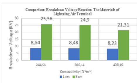
Fig. 4. Comparison breakdown voltage
