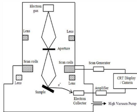
Fig. 3. Scanning Electron Microscope diagram
