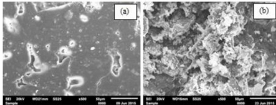
Fig. 13. SEM photos epoxy resin insulating material with silicon rubber filler and silica 50%, respectively (a) RTV 25 referral and (b) RTV 25 aging electricity for 6 minutes
