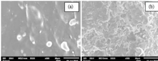
Fig. 12. SEM photos epoxy resin insulating material with silicon rubber filler and silica 40%, respectively (a) RTV 24 referral and (b) RTV 24 aging electricity for 6 minutes
