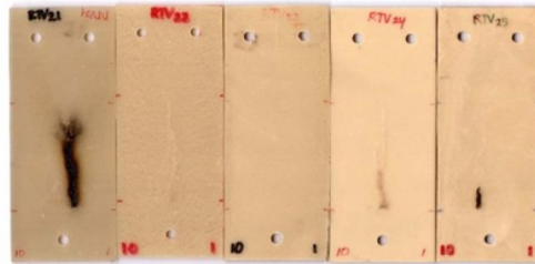
Fig. 8. Surface degradation due to electrical tracking during 6 minutes
