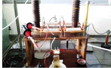
Fig. 5. Inclined Plane Tracking test
