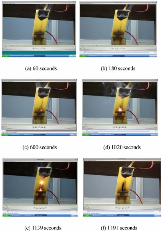
Fig. 7. Step of mechanism of surface tracking
