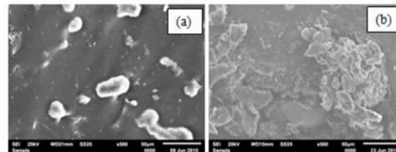
Fig. 9. SEM photos epoxy resin insulating material with silicon rubber filler and silica 10%, respectively (a) RTV 21 referral and (b) RTV 21 aging electricity for 6 minutes
