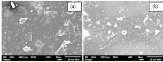
Fig. 11. SEM photos epoxy resin insulating material with silicon rubber filler and silica 30%, respectively (a) RTV 23 referral and (b) RTV 23 aging electricity for 6 minutes
