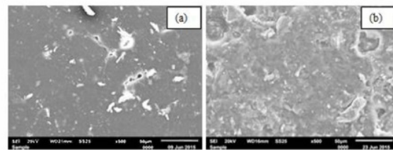
Fig. 10. SEM photos epoxy resin insulating material with silicon rubber filler and silica 20%, respectively (a) RTV 22 referral and (b) RTV 22 aging electricity for 6 minutes
