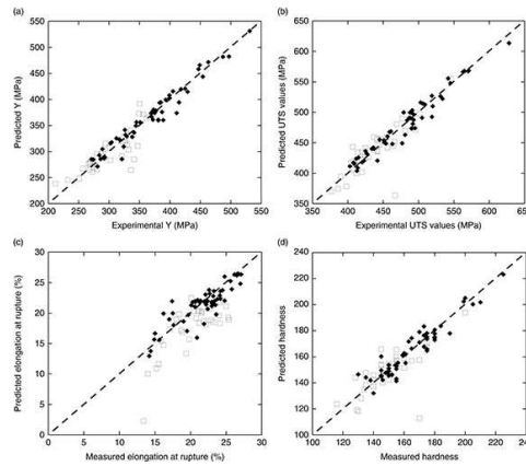
Figure 1. (a) Correlation between predicted and experimental values of Y, (b) UTS, (c) A and (d) HB. Solid symbols refer to fully ferritic alloys, open symbols to those containing more than 2% pearlite.
