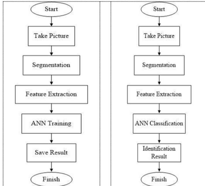
Figure 2. Shows the Training Process stages. Flowchart of Artificial Neural Networks (ANN) Training begins with taking a picture then the segmentation process from the original image is changed to grayscale, then performs feature extraction and training of ANN with neurons, rate, and iteration that has been varied than the weight values will be stored in .mat file which will be tested later.
