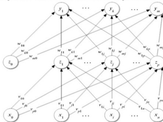
Figure 4. Backpropagation Architecture
