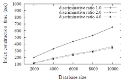
Fig. 2: The scalability of algorithm FMDCS
