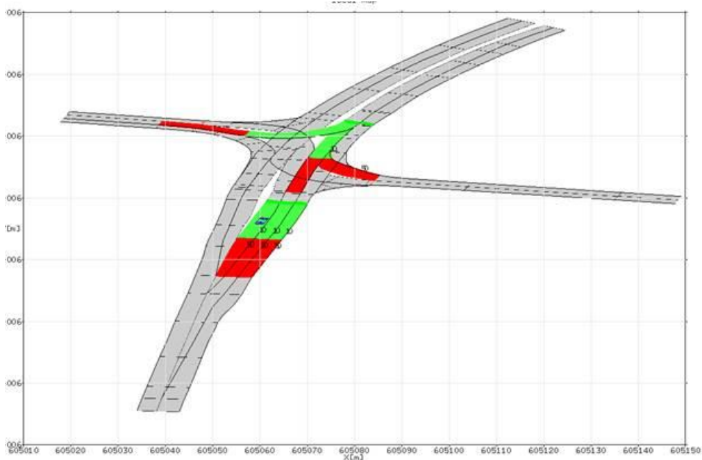
Figure 17: Speed advice visualisation on Tostmannplatz for a subset of lanes.
