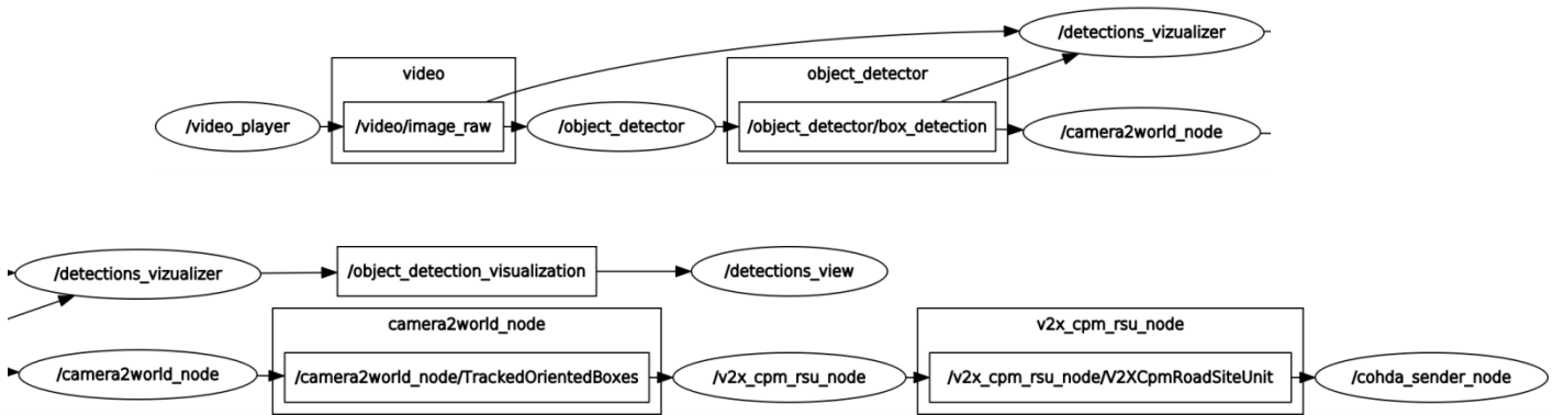
Figure 50: Building blocks of the hemispheric camera to CPM processing pipeline
