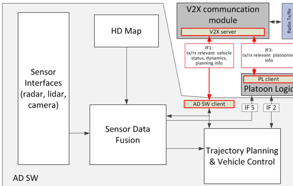
Figure 8: General AD Software modules and MAVEN V2X system integration scheme for V2V platooning communications in the vehicle
