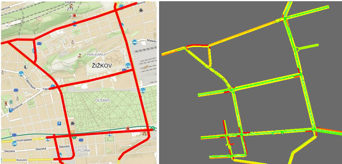
Figure 79: UC12 test polygon at Praha Žižkov (left) and a snapshot of the Eclipse SUMO simulation (right) showing actual link travel delays for the highest (i.e. circa 3600 vph) flow rate settings.
