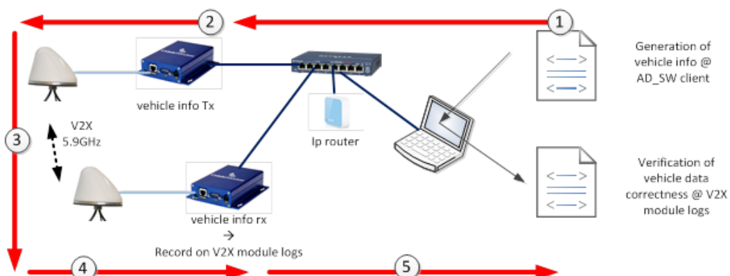
Figure 9: Verification scheme for V2X integration implementation of platooning communications
