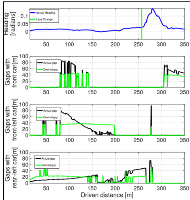
Figure 76: HMETC lance change advice adaptation at the Helmond test intersection (1)
