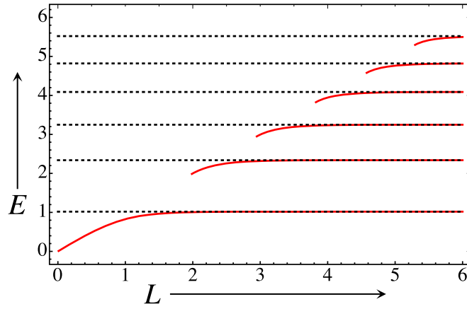
Figure 2. Red curves: even and odd energy levels in the truncated potential (1.2), for increasing truncation distance L ; dotted lines: levels of the untruncated linear potential, i.e. zeros of Ai' (even levels) and Ai (odd levels).
