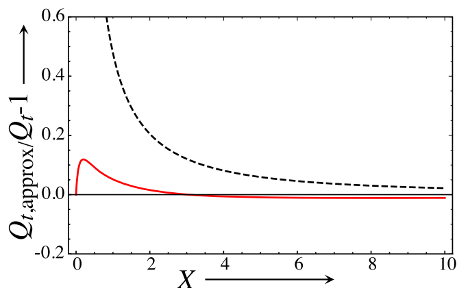
Figure 4. Errors in approximations to the truncation function Q_t . Dashed curve: large X approximation Q_{t,\text{large}} (3.3); red curve: approximation Q_{t,\text{combined}} (3.5) fitting the large and small X limits.
