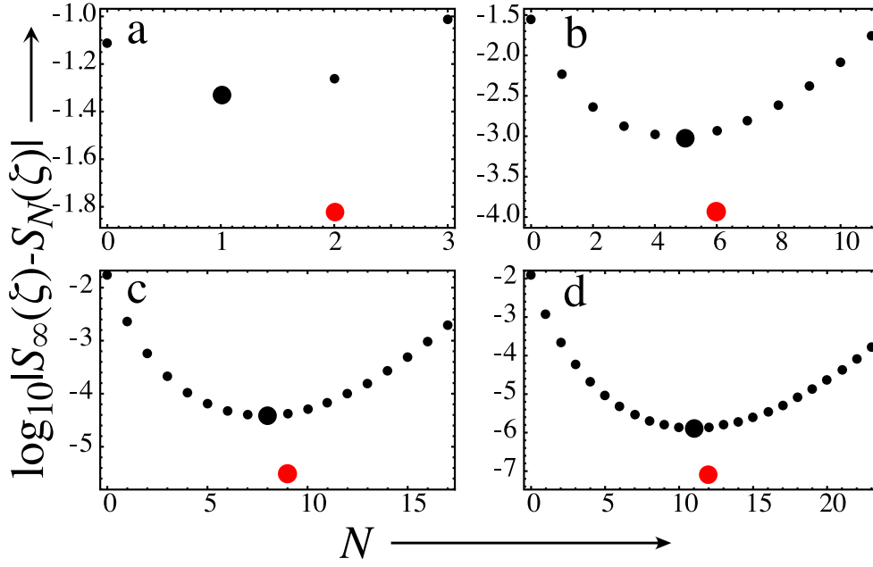
Figure 6. Black dots: errors in the approximations S_N(\zeta(E)) (4.4) to the sum S_\infty(\zeta(E)) (4.8) for successive truncations N , showing the divergence of the series; the large dots indicate the smallest term: N = N_{\text{opt}}(E) . Red dots: errors when the series optimally terminated at N_{\text{opt}}(E) is corrected by the resummed tail R_{\text{summed}}(E) (4.15), for energies E of the four lowest levels of the untruncated potential (1.2): (a) E = 1.019 ( N_{\text{opt}} = 1 ); (b) E = 2.338 ( N_{\text{opt}} = 5 ); (c) E = 3.248 ( N_{\text{opt}} = 9 ); (d) E = 4.008 ( N_{\text{opt}} = 12 ).
