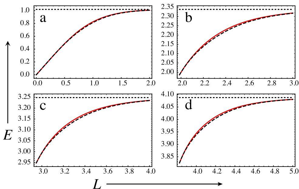
Figure 5. Lowest levels after their appearance when L = L_{\text{birth}} (..) (magnification of part of figure 2); red curves: exact; dashed curves: using the approximation Q_{t,\text{combined}} (3.5); dotted lines, levels of untruncated linear potential (1.2), i.e. zeros of \text{Ai} and \text{Ai}' . (a) Lowest even level (ground state); (b) lowest odd state; (c) first excited even state; (d) first excited odd state.
