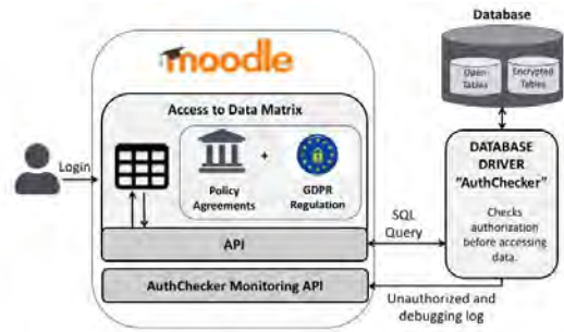
Figure 2: Components and execution flow of the developed solution.
