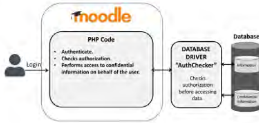
Figure 1: The solution we propose, called AuthChecker.
