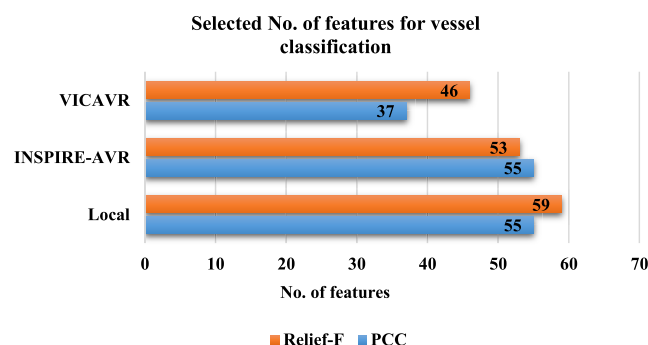
Fig. 18. Feature subsets selected for vessel classification, using two different ranking methods for VICAVER, INSPIRE-AVR and Local database.
