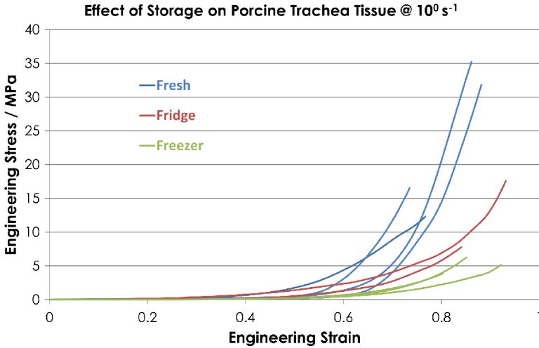
Fig. 2. Stress–strain data of porcine trachea samples. See text for details on sample size and measurements.
