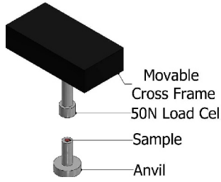
Fig. 1. Three-dimensional schematic image of the key components of the Instron screw-driven press. Biological samples were placed on the lightly-lubricated top surface of the stationary anvil. A load cell, certified to 50 N in the case of these experiments, attached to a movable cross frame is used to compress the sample at a pre-selected strain rate. The apparatus is controlled and data is extracted using BlueHill software running on a Windows PC.
