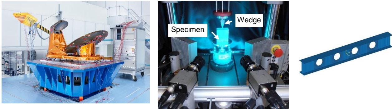
Figure 1: Exemplars of the validation ILS: a full CFRP space antenna reflector (left); wedge indenter deforming a rubber block (experimental arrangement) (centre); and an I-beam with holes under 3-point bending (simulation model) (right).
