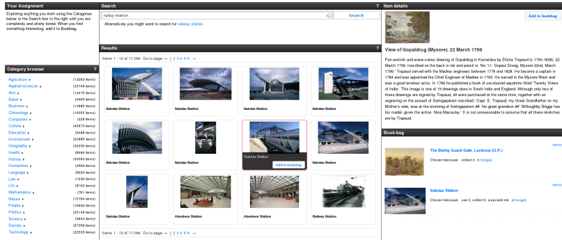
Fig. 2. Screenshot showing the task UI used in the experiments. The UI consists of six parts. On the left are the task instructions and the category browser. In the middle are the search box and the search results. On the right are the viewer for an item's details and the book-bag used to store interesting items. Selecting a category on the left, entering search terms, or clicking on a meta-data facet in the item viewer all resulted in the items matching that request being displayed in the central 4 \times 3 grid.
