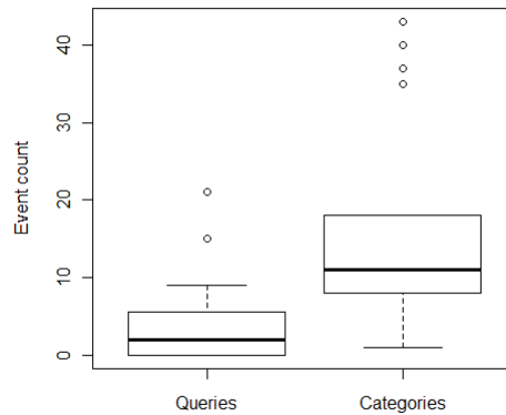
Fig. 6. Comparison of query and category select counts
