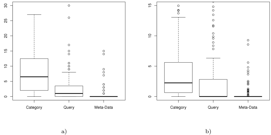
Fig. 4. Box-plots showing: a) the number of interactions in each of the three exploration methods; b) the amount of time (in minutes) spent on each of the three exploration methods. “Category” refers to using the category browser, “Query” to typing a query into the search box, and “Meta-Data” to exploring the collection by clicking on the meta-data facets shown in the item viewer.
