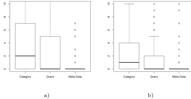
Fig. 5. Box-plots showing: a) the number of items viewed ; b) the number of items saved to the book-bag when using each of the exploration methods. “Category” refers to using the category browser, “Query” to typing a query into the search box, and “Meta-Data” to exploring the collection by clicking on the meta-data facets shown in the item viewer.
