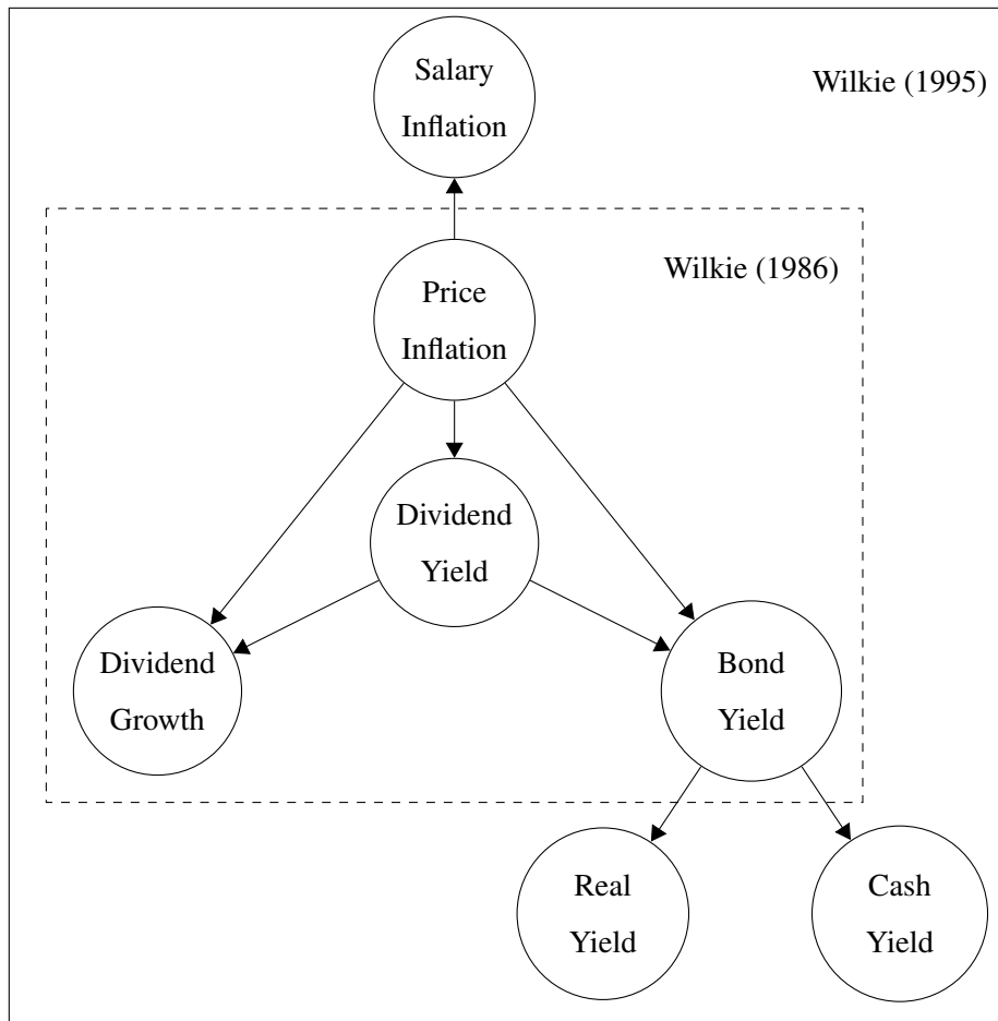
Figure 2.1: Wilkie Models: Cascade structure.
