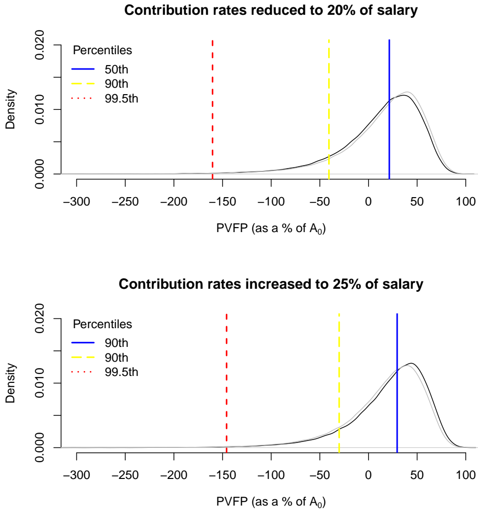
Figure 5.3: Distributions of standardised PVFP (as a percentage of A_0 = \pounds 41.6\text{bn} ) for decreased contribution rate of 20% and increased contribution rate of 25% (base case assumption is 22.5% of salary) using Graphical Model. The grey coloured density in the background shows the base case.
