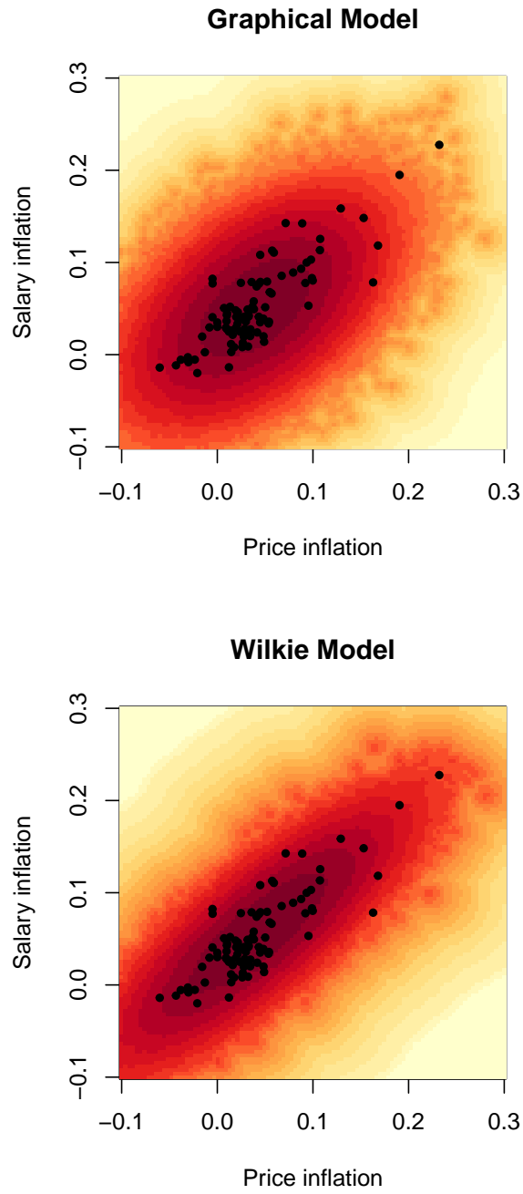
Figure 2.10: Plots of simulated price and salary inflation from the UK Graphical Model and the Wilkie Model, where the black dots represent historical observations.
