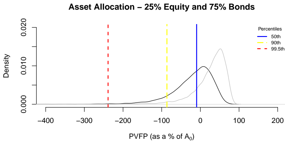
Figure 7.2: Distributions of standardised PVFP (as a percentage of A_0 = \$227.5\text{bn} ) for asset allocation strategy. Base case distribution is superimposed in grey for comparison.
