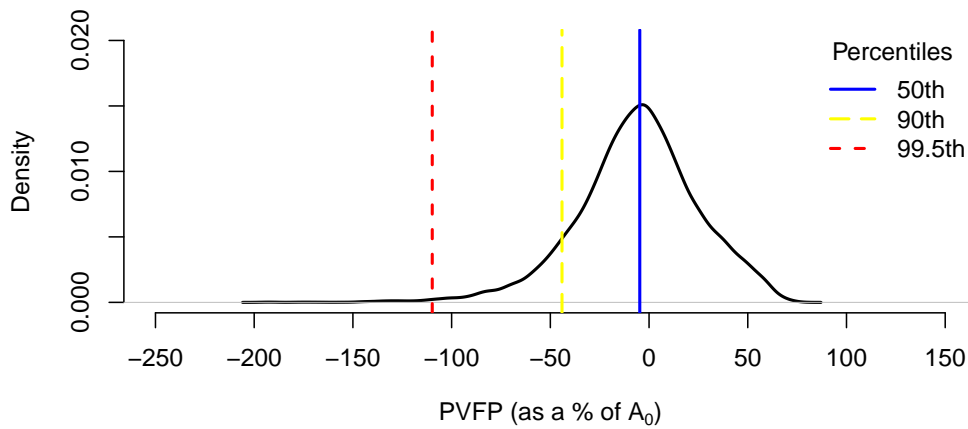
Figure C.2: Distributions of standardised PVFP (as a percentage of A_0 ) for the base case and for the asset allocation strategy of 30% equities and 70% bonds at different probability levels using the Graphical model.
