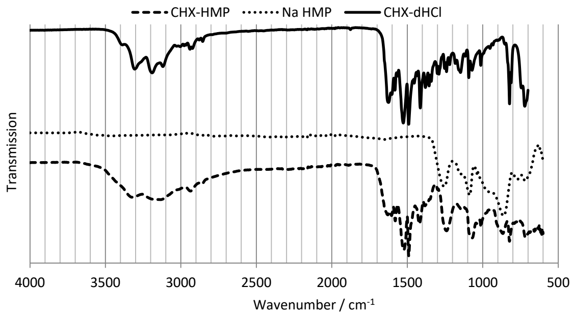
Figure 2. FT-IR spectra of CHX-HMP, sodium hexametaphosphate (Na HMP) and chlorhexidine dihydrochloride (CHX-dHCl)
