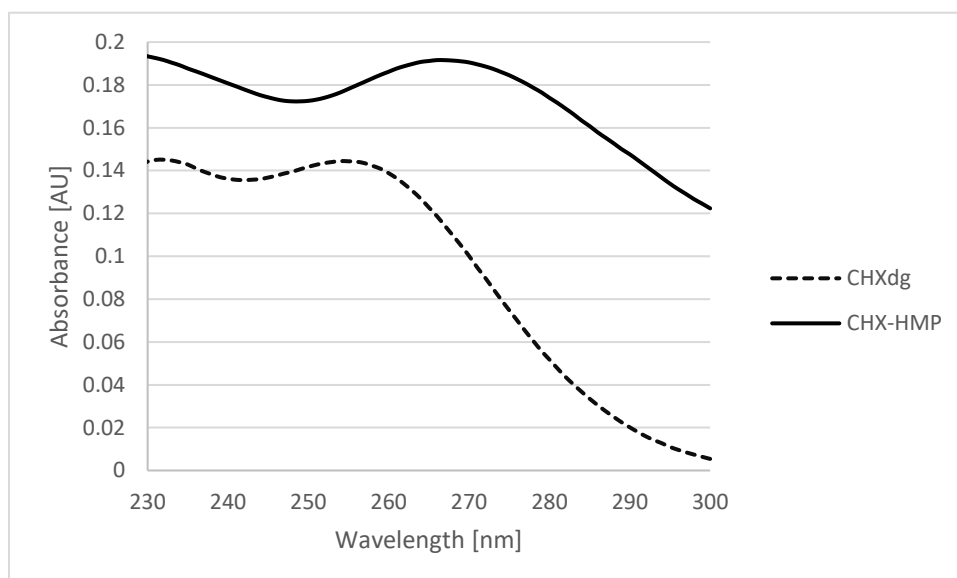
Figure 1. UV absorption spectra of CHXdg solution and CHX-HMP suspension. There is a bathochromic shift in the first absorption maximum following the precipitation reaction, from 254 nm for CHXdg to 268 nm for CHX-HMP.
