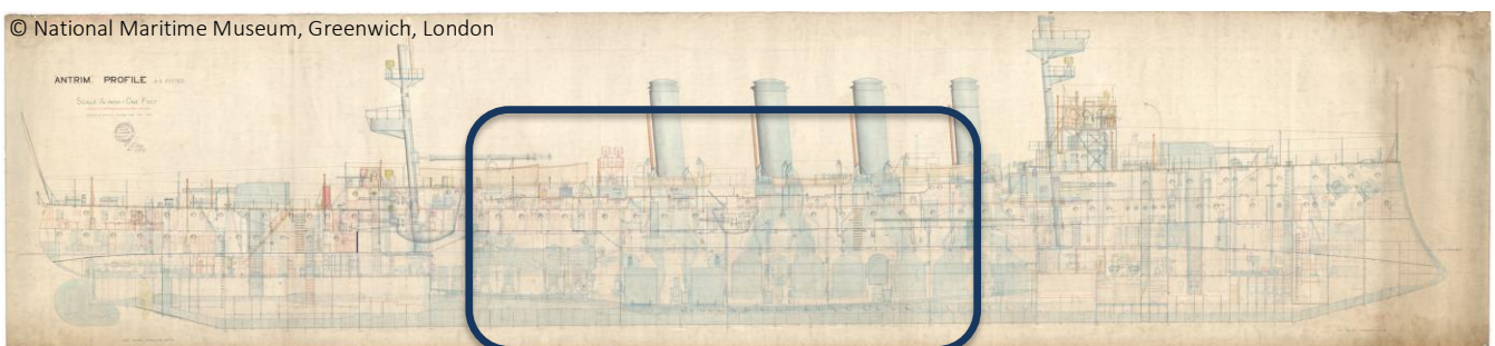
Figure 67: Plan Amidships
