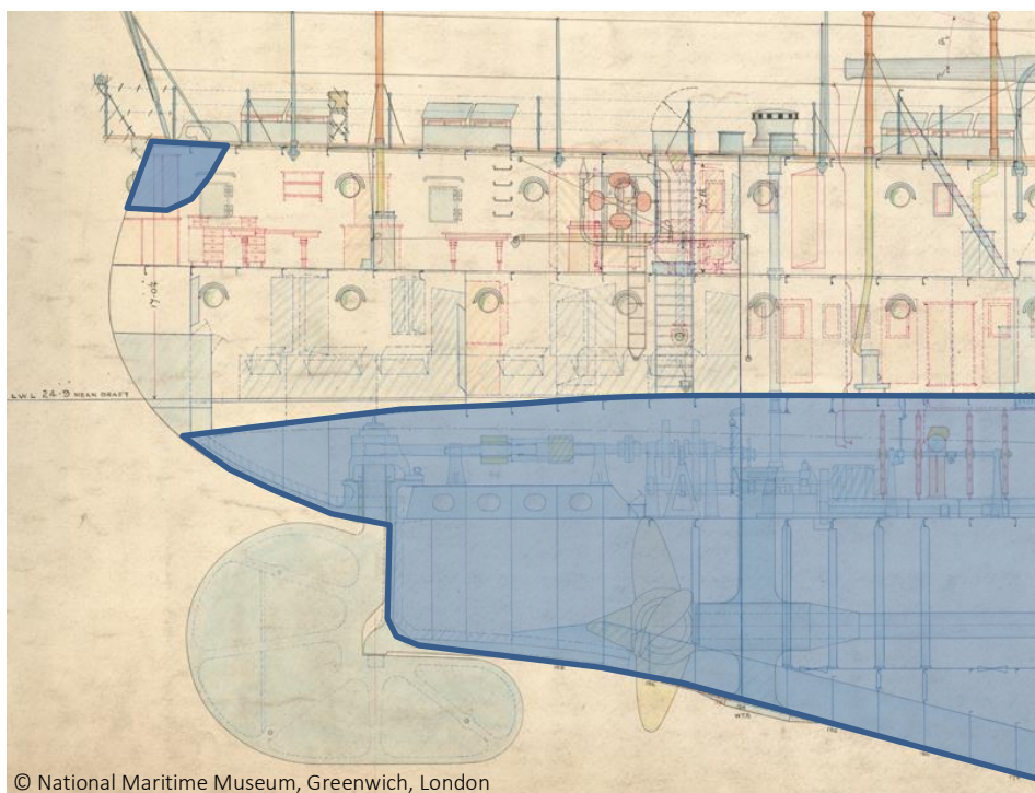
Figure 97: Plan of stern section, highlighting remaining intact structure
