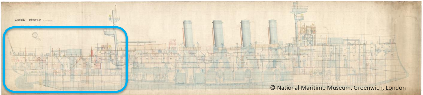
Figure 83: The stern section of HMS HAMPSHIRE as surveyed extends from just forwards of the aft casemate at approximately frame No 145 to the stern encompassing the aft 7.5 inch turret, rudder and her one remaining propeller and shaft
