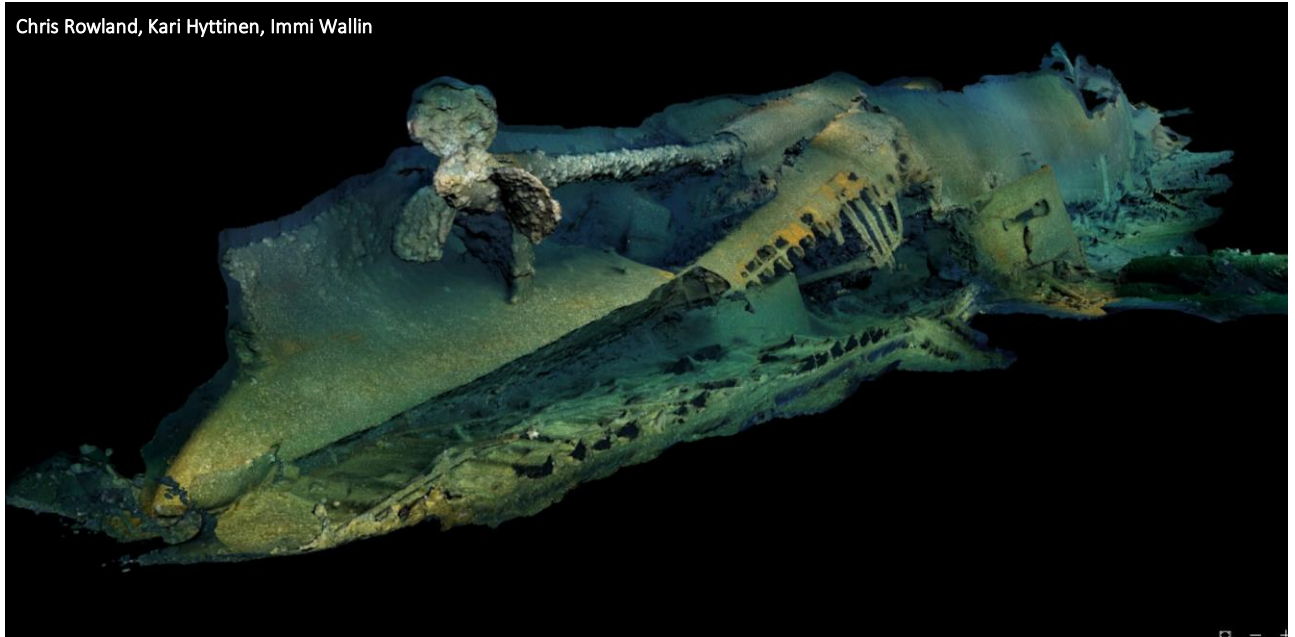
Figure 30: Dense point cloud of the stern section
