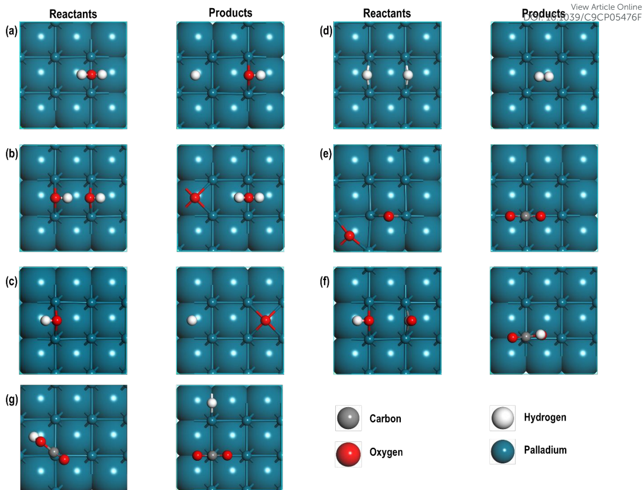
Figure 3. The top view of reactants and products of (a) water splitting, (b) Formation of \text{H}_2\text{O} and adsorption of O, (c) OH splitting, (d) \text{H}_2 evolution, (e) CO oxidation, (f) Formation of carboxyl species and (g) \text{CO}_2 evolution from carboxyl species. For clarity the upper most atomic layer is shown in ball and stick and lower sub-surfaces are shown in van der Waals representation.
