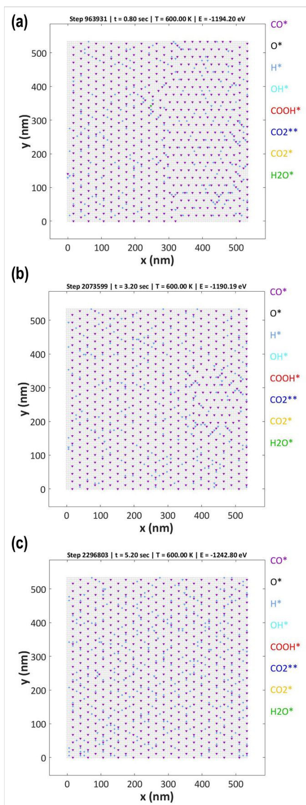
Figure 8. Snapshots for simulation area at (a) 0.8 s, (b) 3.2 s and (c) 5.2 s. All simulation have 1 to 1 ratio for H 2 O and CO in the gas phase, under the conditions stated in computational details section.
