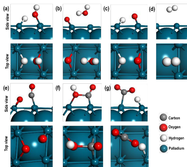
Figure 5. Top and side views of (a) TS1, (b) TS2, (c) TS3, (d) TS4, (e) TS5, (f) TS6, and (g) TS7 where, TS represents transition states and 1 – 7 represents the steps. For clarity the upper most atomic layer is shown in ball and stick and lower sub-surfaces are shown in van der Waals representation.
