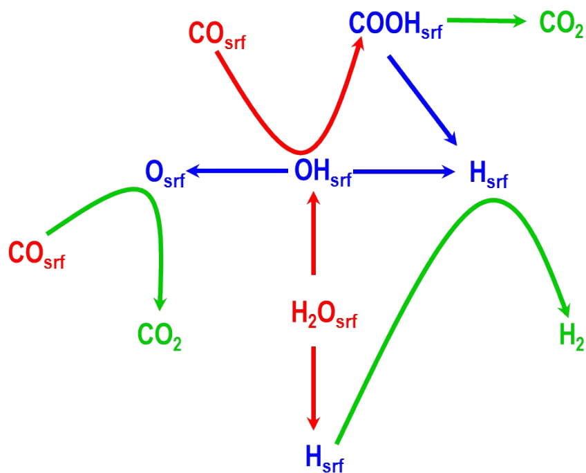
Figure 1. A mechanism consisting of seven core elementary steps involving both redox and carboxyl mechanisms for water gas shift reaction. For simplicity the adsorption and desorption steps are not shown.
