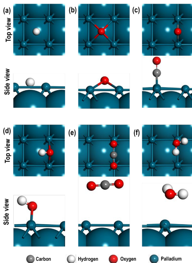
Figure 2. Top and side views of the most stable structures of (a) H atom, (b) O atom, (c) CO molecule, (d) OH species, (e) CO 2 molecule, and (f) H 2 O molecule. For clarity the uppermost layer is shown as ball and stick format and for the lower subsurfaces van der Waals representation of the atoms is adopted.
