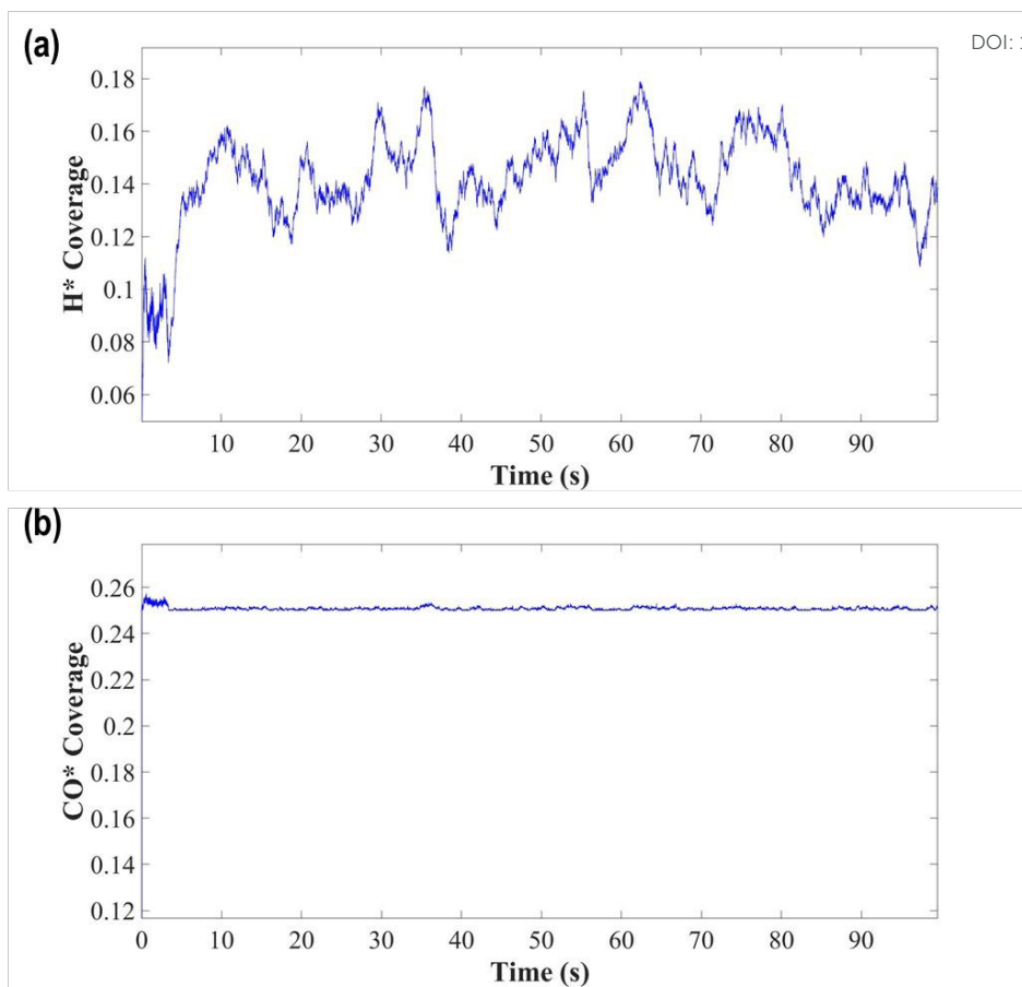
Figure 7. (a) H and (b) CO coverage against time
