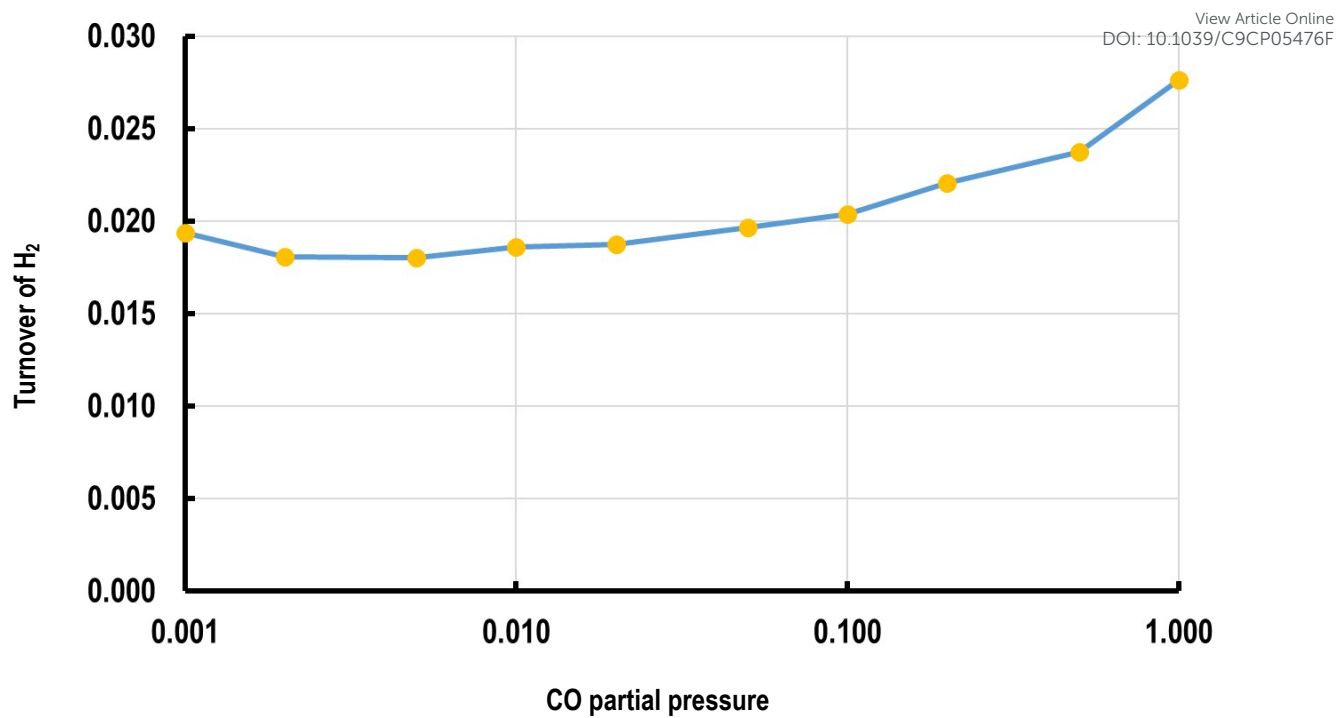
Figure 9. Plot of turnover frequency for H 2 against the ratio of H 2 O/CO partial pressure.
