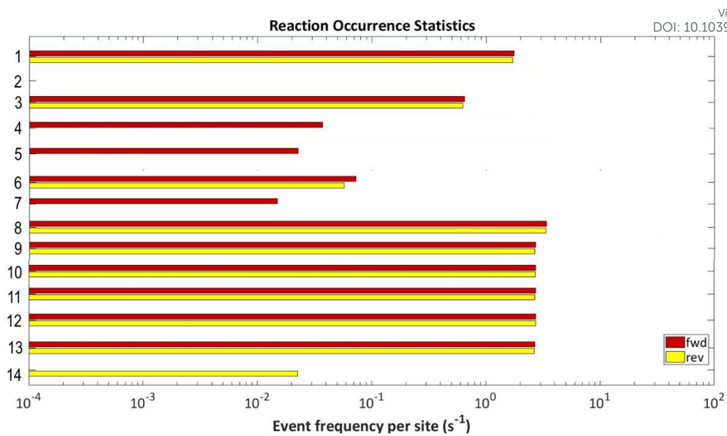
Figure 10. Event frequency per site for each of the elementary steps of the proposed reaction mechanism.
