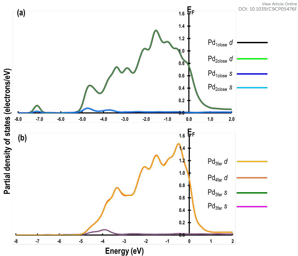
Figure 4. Partial density of states for (a) Pd atoms in close proximity and (b) Pd atoms further away from the adsorbed O-atom.
