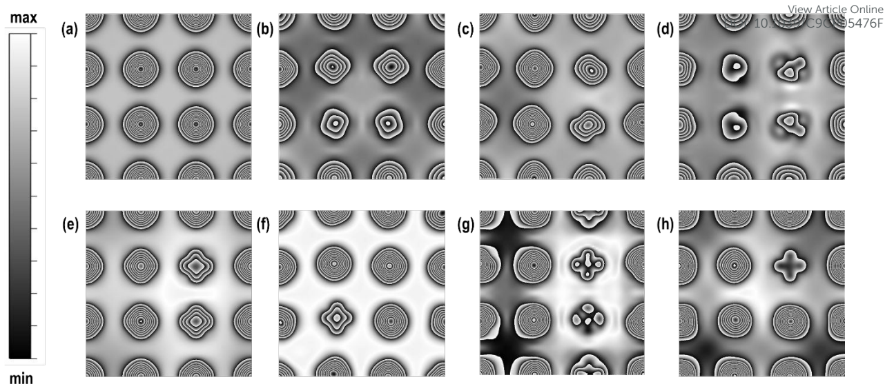
Figure 6. Spin densities of the exposed surface in (a) pristine Pd(100) ( \text{min}=9.45 \times 10^{-7} \text{ e}/\text{\AA}^3 , \text{max} = 4.13 \times 10^{-5} \text{ e}/\text{\AA}^3 ) and during the interaction of the transition states in (b) Step 1 ( \text{min}=7.63 \times 10^{-7} \text{ e}/\text{\AA}^3 , \text{max} = 2.79 \times 10^{-5} \text{ e}/\text{\AA}^3 ), (c) Step 2 ( \text{min}=4.44 \times 10^{-7} \text{ e}/\text{\AA}^3 , \text{max} = 3.37 \times 10^{-5} \text{ e}/\text{\AA}^3 ), (d) Step 3 ( \text{min}=5.52 \times 10^{-8} \text{ e}/\text{\AA}^3 , \text{max} = 1.80 \times 10^{-5} \text{ e}/\text{\AA}^3 ), (e) Step 4 ( \text{min}=-1.68 \times 10^{-7} \text{ e}/\text{\AA}^3 , \text{max} = 2.74 \times 10^{-5} \text{ e}/\text{\AA}^3 ), (f) Step 5 ( \text{min}=-3.22 \times 10^{-5} \text{ e}/\text{\AA}^3 , \text{max} = 5.89 \times 10^{-3} \text{ e}/\text{\AA}^3 ), (g) Step 6 ( \text{min}=-7.71 \times 10^{-8} \text{ e}/\text{\AA}^3 , \text{max} = 4.69 \times 10^{-6} \text{ e}/\text{\AA}^3 ) and (h) Step 7 ( \text{min}=-3.04 \times 10^{-8} \text{ e}/\text{\AA}^3 , \text{max} = 1.02 \times 10^{-5} \text{ e}/\text{\AA}^3 ).
