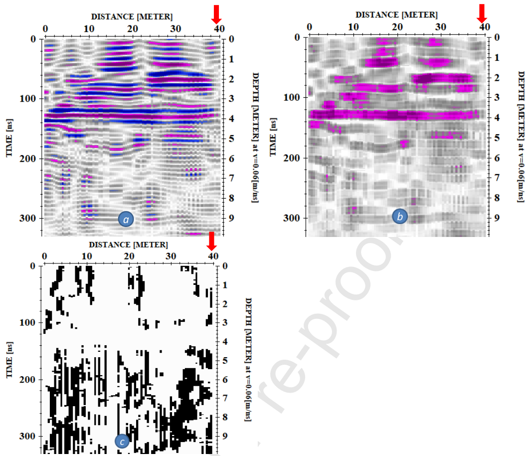
Fig.12 GPR profile after conventional processing (a), the average amplitude attribute (b) and the coherence attribute (c) of the depression data. The red arrows indicate the auger position corresponding to radar images.
