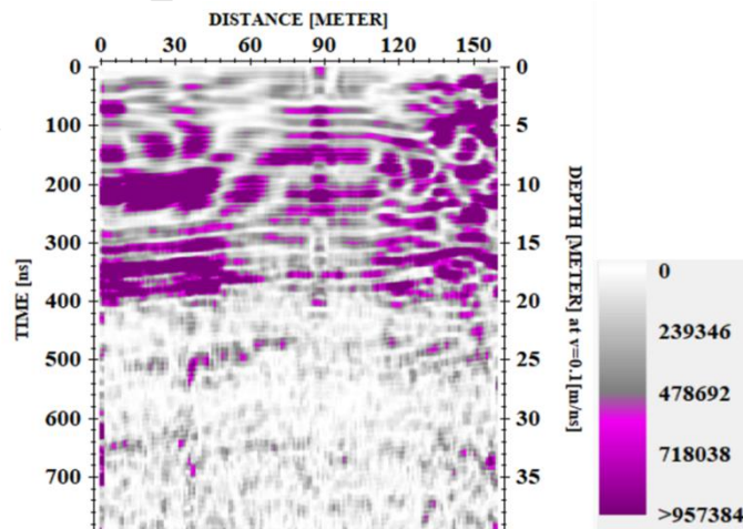
Fig.7 Average energy attribute image of demonstration data and associated colour bar; the bright purple part represents high energy of the signal and the grey and white colour parts reflect low energy.
