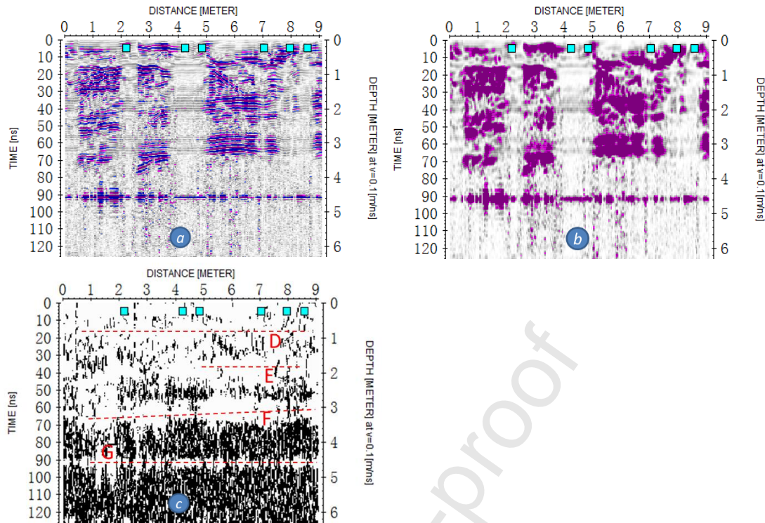
Fig.11 GPR profile images after conventional processing (a), the average energy attribute (b) and the coherence attribute (c) of No.2 epikarst profile. The block markers in the figures are corresponding to small red flags except both ends in Fig.3. The letters D, E, F, G and dotted lines indicate the layers' general position.
