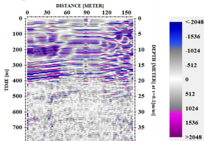
Fig.6 Radar image of exemplar site following conventional data processing, with accompanying colour bar; purple represents strong positive amplitude and blue represents strong negative amplitude; dim grey and white colours
