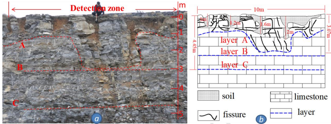
Fig.2 Photograph (a) and sketch map (b) of No.1 epikarst profile
