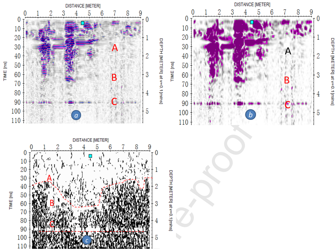
Fig.10 GPR profile images after conventional processing (a), the average energy attribute (b) and the coherence attribute (c) of No.1 epikarst profile. The block markers correspond to the position marked by the hammer in Fig.2.
