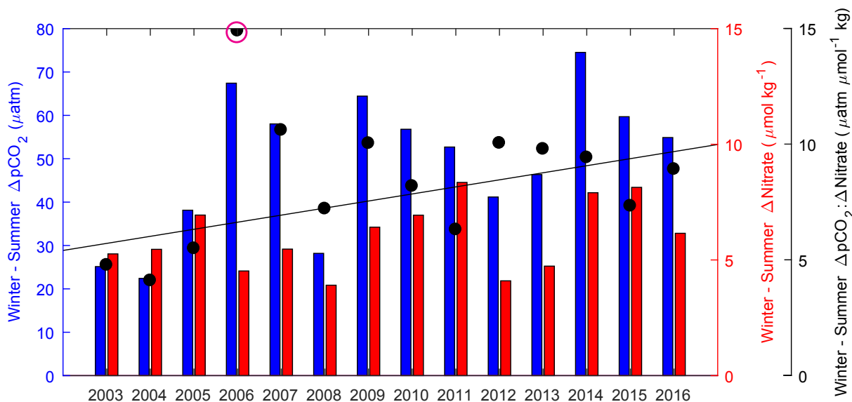
Fig. 4. The annual difference between winter maximum and summer minimum seawater pCO_2 (nitrate) represented by the blue (red) bars and shown on the left (right) vertical axis. The ratio of \Delta pCO_2 to \Delta Nitrate is represented by the black symbols and shown on the secondary right vertical axis. One outlier was removed from the long term trend analysis.
