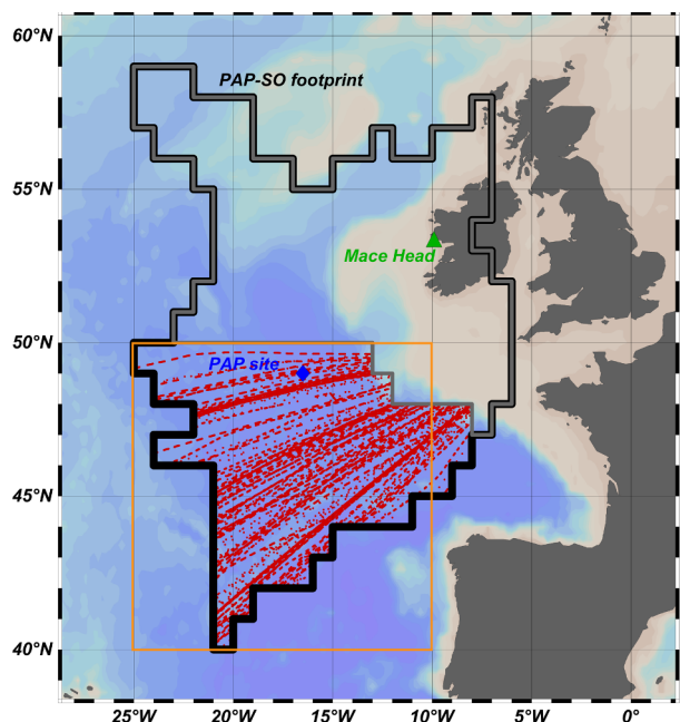
Fig. 1. Map of the study area showing all pCO 2 measurement locations in red symbols, the PAP footprint as the black contour, the excluded area as the grey contour, the location of the mooring at the PAP-SO site as the blue diamond and Mace Head atmospheric observatory as the green triangle. The orange box shows the extent of the NPP data selected. Produced with Ocean Data View (Schlitzer, 2016).
