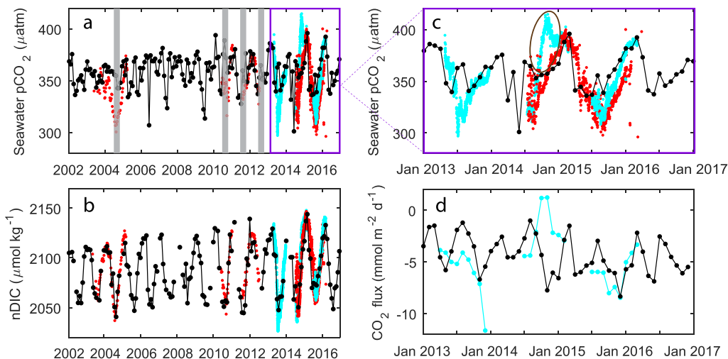
Fig. 5. (a) Comparison between the spatially and temporally-averaged pCO_2 from the SOO (black symbols) and the pCO_2 recorded by the 1 m (cyan symbols) and 30 m depth (red symbols) sensors on the PAP buoy. Grey bars cover months when the 30 m sensor is outside the mixed layer (b) Same as above, but for salinity-normalised DIC. (c) Zoom-in on the 2013–2016 period in sub-figure a. The period where the 1 m sensor was affected by a storm is shown in the brown oval. (d) Comparison between the CO_2 flux calculated using the SOO pCO_2 and the flux calculated with monthly-averaged PAP 1 m sensor pCO_2 .
