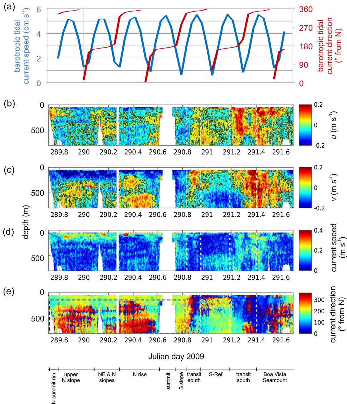
Fig. 7. Same as Fig. 6, but for the time interval of the transition from Senghor Seamount to S-Ref and further south to the Boa Vista Seamount. Note the layered internal-wave structure in current directions (dashed-line box) and speeds while barotropic tidal current speeds peak at >4.5 \text{ cm s}^{-1} during their semidiurnal cycles. Also note that these internal waves became less obvious after the ship had left the seamount on day 290.85 while barotropic tidal current speeds still peaked at >4.5 \text{ cm s}^{-1} during their semidiurnal cycles.
