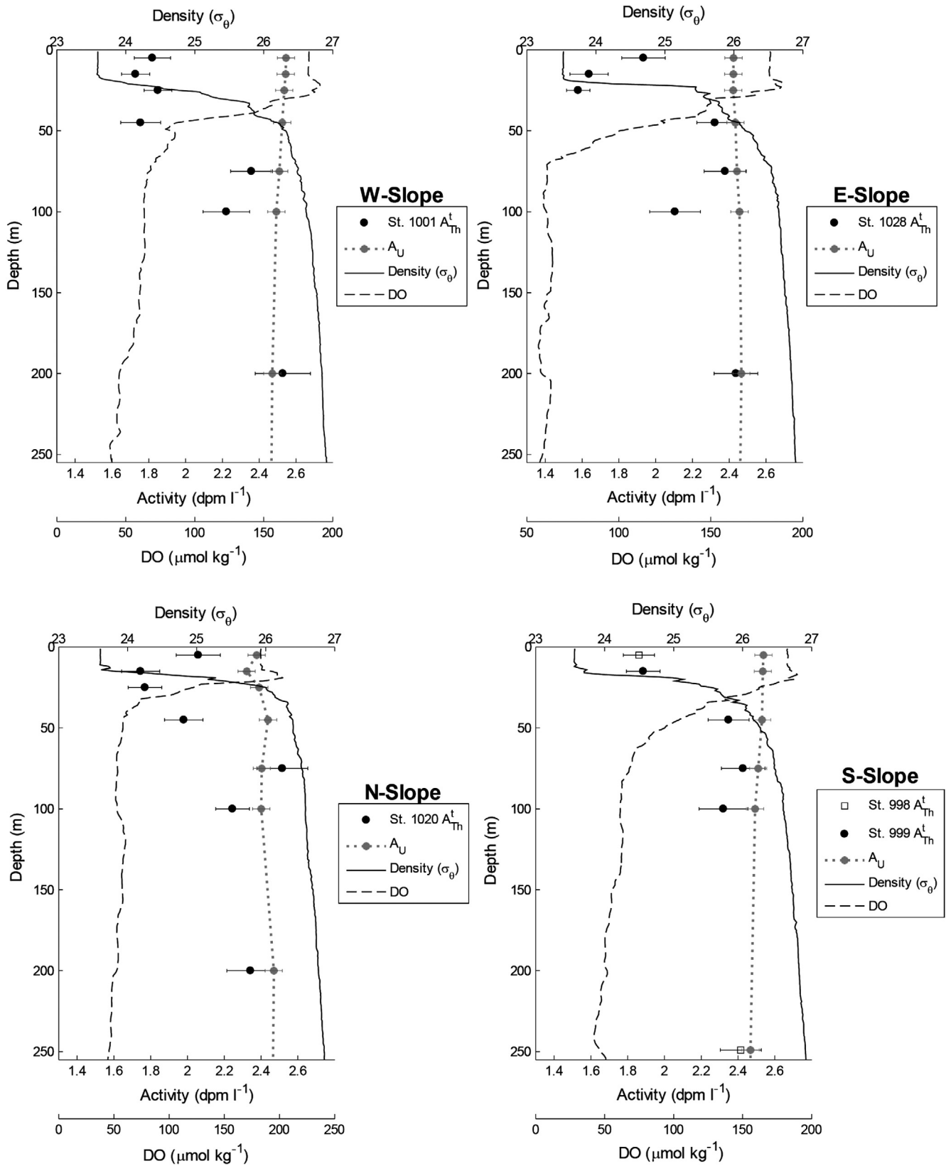
Fig. 11. Same as Fig. 10, but for the W-Slope (top-left), E-Slope (top-right), N-Slope (bottom-left) and S-Slope (bottom-right).
