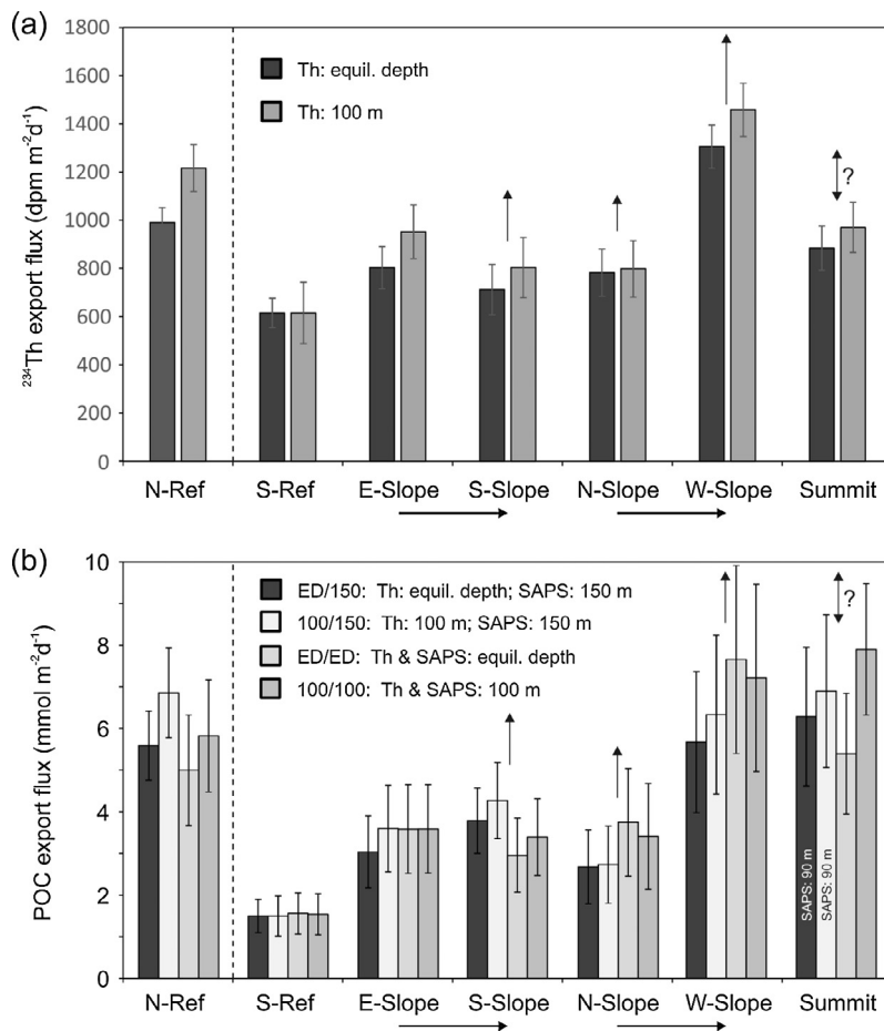
Fig. 12. (a) Export fluxes of ^{234}\text{Th} . Results for two different ways of calculating the fluxes are shown. (b) Export fluxes of POC. Results for four different ways of calculating the fluxes are shown. N-Ref is not viewed as a suitable reference site and separated from the other station results by the vertical dashed line. S-Ref was a suitable reference site for the seamount stations. Horizontal arrows below abscissa: E-Slope and N-Slope are viewed as sites that are located approximately upstream of S-Slope and W-Slope, respectively. Upward arrows indicate probable underestimates. Bidirectional arrow with '?': here, it is unclear whether there is an under- or overestimate. Error bars: \pm one propagated standard deviation.
