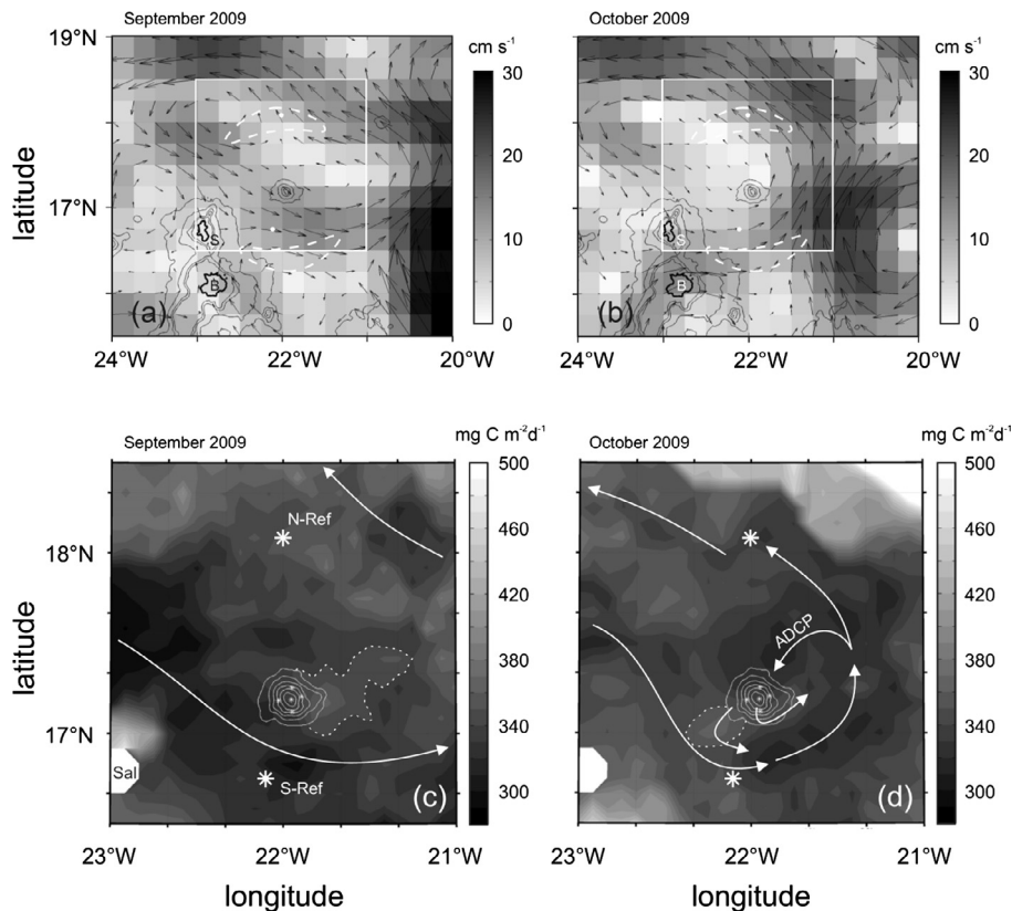
Fig. 2. (a) AVISO-derived surface currents during September 2009. Bold isobaths: outlines of Sal island (S) and Boa Vista island (B). Areas surrounded by dashed white lines: approximate regions where the initial downward semidiurnal internal-tide beams that are generated on the upper slopes of Senghor Seamount reflect from the sea surface (also see Fig. S3). White circles: locations of N-Ref and S-Ref. Area surrounded by white rectangle line: area shown in (c) and (d). (b) Same as (a), but for October 2009. (c) Map of net primary productivity (NPP) in September 2009 as derived from the Vertically Generalized Productivity Model (VGPM; Behrenfeld and Falkowski, 1997). White approximately concentric lines: approximate outline of Senghor Seamount. White star symbols: sampling sites. White arrows: approximate (hand-drawn) AVISO-derived surface currents. The area that is surrounded by a thin white dashed line and emanates from the seamount indicates what could be a 'banner cloud' of seamount-enhanced NPP on the downstream side of the seamount. (d) Same as (c), but for October 2009. The detail of the approximate hand-drawn currents labelled 'ADCP' is derived from the VM-ADCP survey as shown in Fig. 3.
