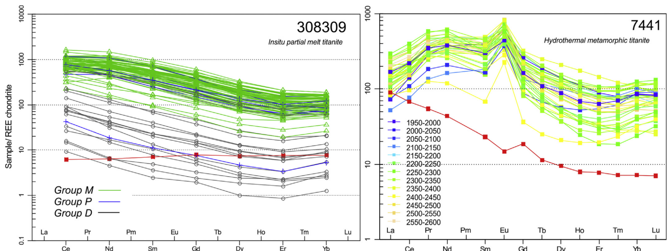
Fig. 9. Chondrite normalized REE plots of titanite from 308309 (left) and 7441 (right). Whole rock REE pattern denoted by red trace (note for 308309 this reflects the leucosome absent component). 308309 is coloured according to interpreted titanite groups. 7441 is colour scaled according to 207-corrected date (in Ma). (For interpretation of the references to colour in this figure legend, the reader is referred to the web version of this article.)
