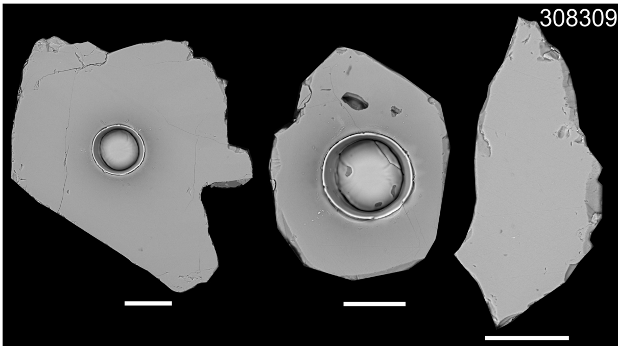
Fig. 3. Backscatter electron image of representative titanite grains from sample 308309 migmatitic amphibolitic gneiss, Akia Terrane, Greenland. Scale bars are 50 \mu\text{m} . Two grains show laser ablation craters.
