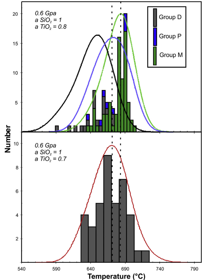
Fig. 10. Upper, Combined histogram and probability plot of Zr-in-titanite temperatures (°C) for the different titanite groups in sample 308309. The higher temperatures in this distribution are interpreted to more likely reflect formation temperatures due to post crystallization alteration in Groups P and D. Lower, Combined histogram and probability plot of Zr-in-titanite temperatures (°C) for titanite in sample 7441.
