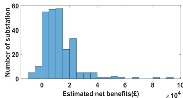
Fig. 12. The distribution of mean net benefits for suburban networks from phase balancing by EQU18
