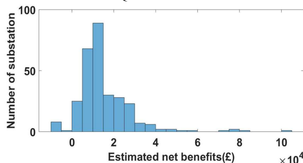
Fig. 11. The distribution of mean net benefits for rural networks from phase balancing by EQU18
