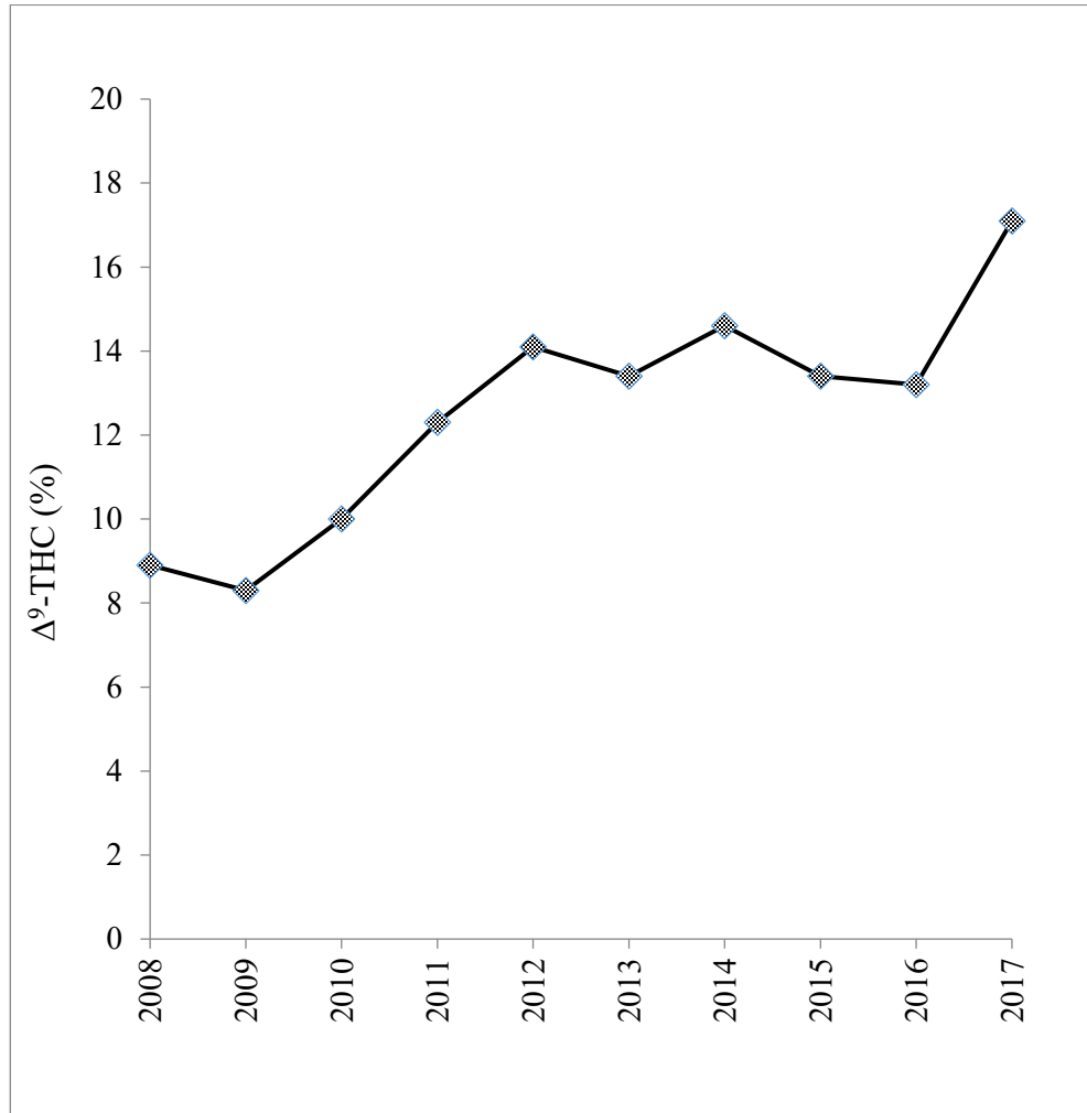
Fig 2 Mean Δ 9 -THC concentration for all samples seized from 2008 to 2017
