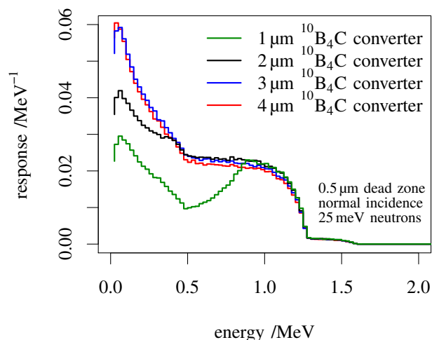
Fig. 4: Neutron response with a 0.5\mu\text{m} dead zone
