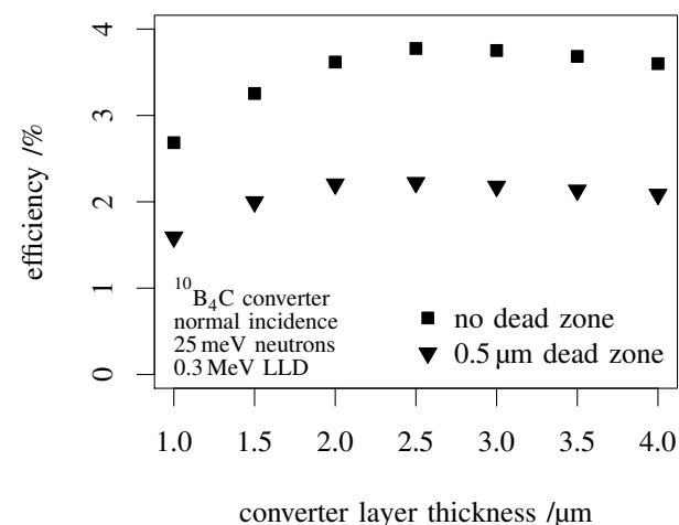
(b) Intrinsic efficiency, 0.3 MeV lower limit of detection
