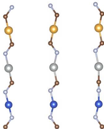
FIG. 11. Left to right: Schematic illustration of the different localized cyanide-rotation modes for a single chain occurring at \sim 38 , 42 and 52 meV, respectively. On the left, all the metal atoms retain their linear connections to C/N, whereas in the center, the Cu and Ag configuration becomes bent. As shown, these two vibrations clearly have different energies. However, once the wave vector possesses a z -component (along the chain), the motions of the cyanide ligands along the chain will have a different relative phase and hence, for a single chain, these two types of motion will resemble one another more and have similar energies. In the right-hand mode, only the cyanide ligands bonded to Au are rotating resulting in a bend in the Au connectivity and hence this mode is higher in energy. Key: Cu, blue, Ag, silver, Au, yellow, C, brown, N, grey.
