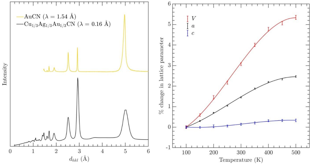
FIG. 2. Left: Synchrotron-based x-ray diffraction (XRD) pattern of \text{Cu}_{1/3}\text{Ag}_{1/3}\text{Au}_{1/3}\text{CN} measured at 100 K, compared to that of commercial AuCN measured at room temperature, using a Bruker D8 diffractometer equipped with primary Cu K_{\alpha 1} radiation. \text{Cu}_{1/3}\text{Ag}_{1/3}\text{Au}_{1/3}\text{CN} is single phase and clearly adopts the AuCN structure. Right: The temperature dependence of the percentage change in the lattice parameters from a Pawley refinement of the synchrotron-based XRD measurements. The points are fitted with an asymmetric sigmoid function.
