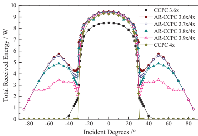
Fig. 8. A comparison of the total received energy of the AR-CCPC with the totally reflective CCPC.
