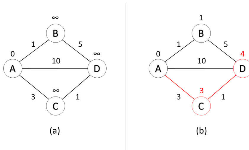
Figure 2.3: Dijkstra process, (a) Initial state, (b) Final state
