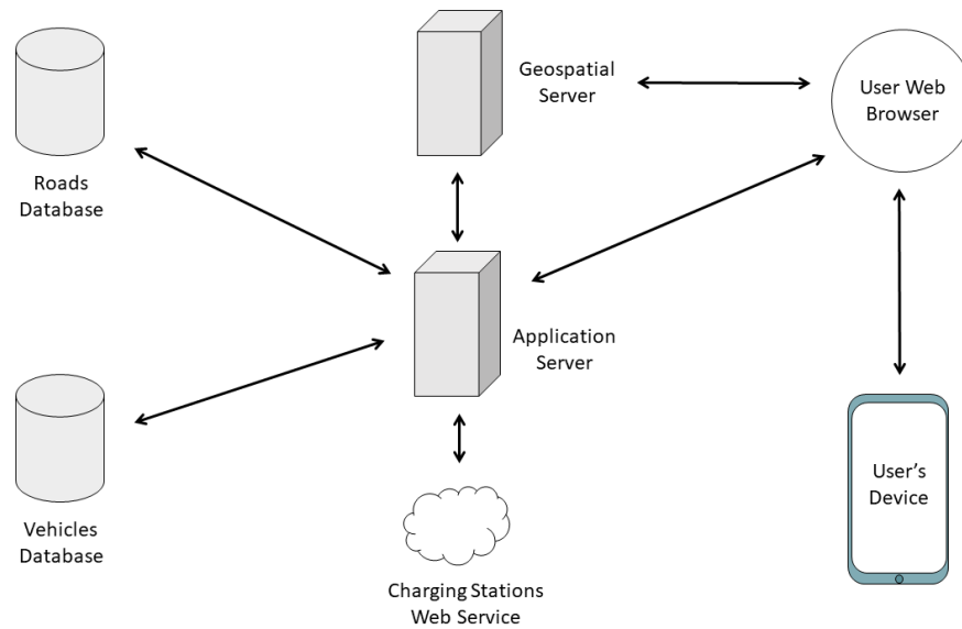
Figure 3.2: Navigation System Workflow. Arrows indicate the direction of the communication
