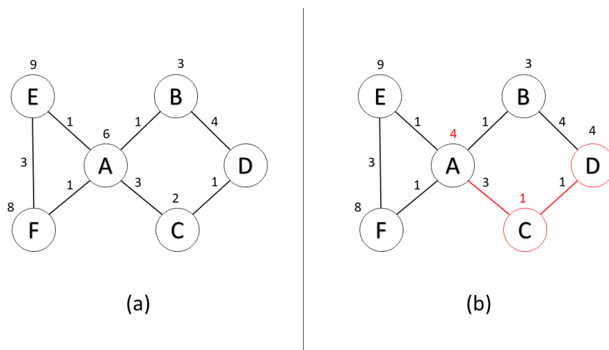
Figure 2.4: A* process, (a) Initial state, (b) Final state
