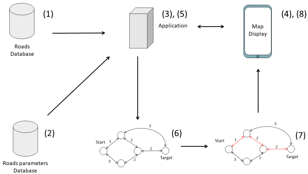
Figure 2.5: Basic Navigation System Workflow
