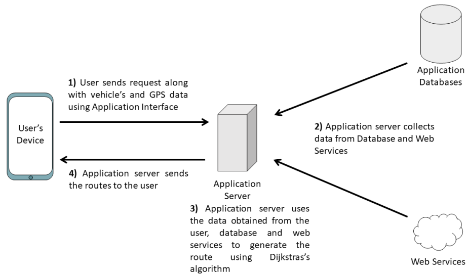
Figure 3.1: General Navigation System Workflow. Arrows indicate the direction of the communication
