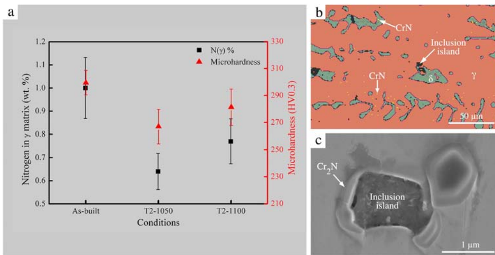
Fig. 11. (a) Changes of nitrogen concentrations in the \gamma matrix ( \text{N}(\gamma)\% ) and microhardness of the as-built, T2-1050 and T2-1100 conditions ( \text{N}(\gamma)\% was measured by EDS detector and at least three points were taken for every sample), (b) EBSD phase diagram for the T2-1050 sample showing the austenite (ochre), ferrite (cyan), CrN (yellow) and inclusions (black), (c) rod-like \text{Cr}_2\text{N} precipitations around the inclusion island after condition T2-1100. (STEDVP was chosen for the calculation of error bars).
