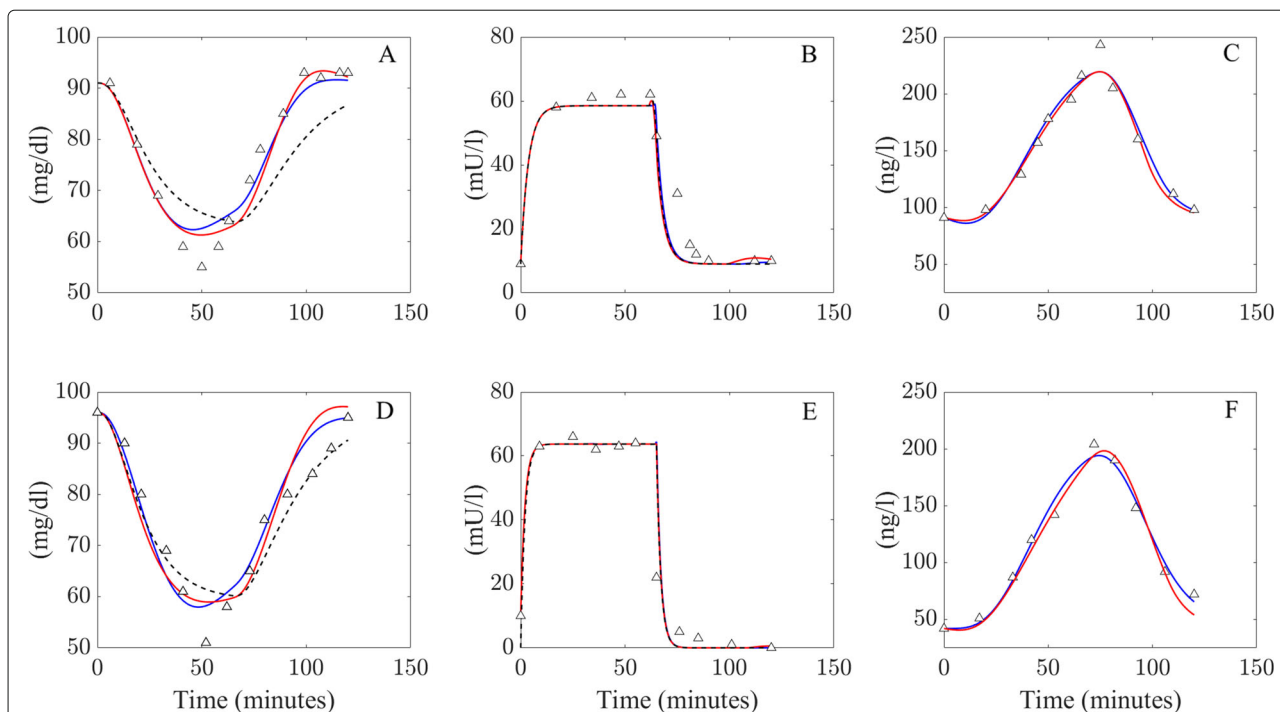
Fig. 3 Model simulations produced from both the LGMM and NLGMM for the insulin induced hypoglycemic tests conducted by [25]. A, B and C shows the predictions for the control group, while D, E and F depicts the results for the diabetic group. Blue lines correspond to solutions from the LGMM, red lines to solutions from the NLGMM and the black dashed lines to the Minimal Model. Experimental data from [25] is shown as triangles
