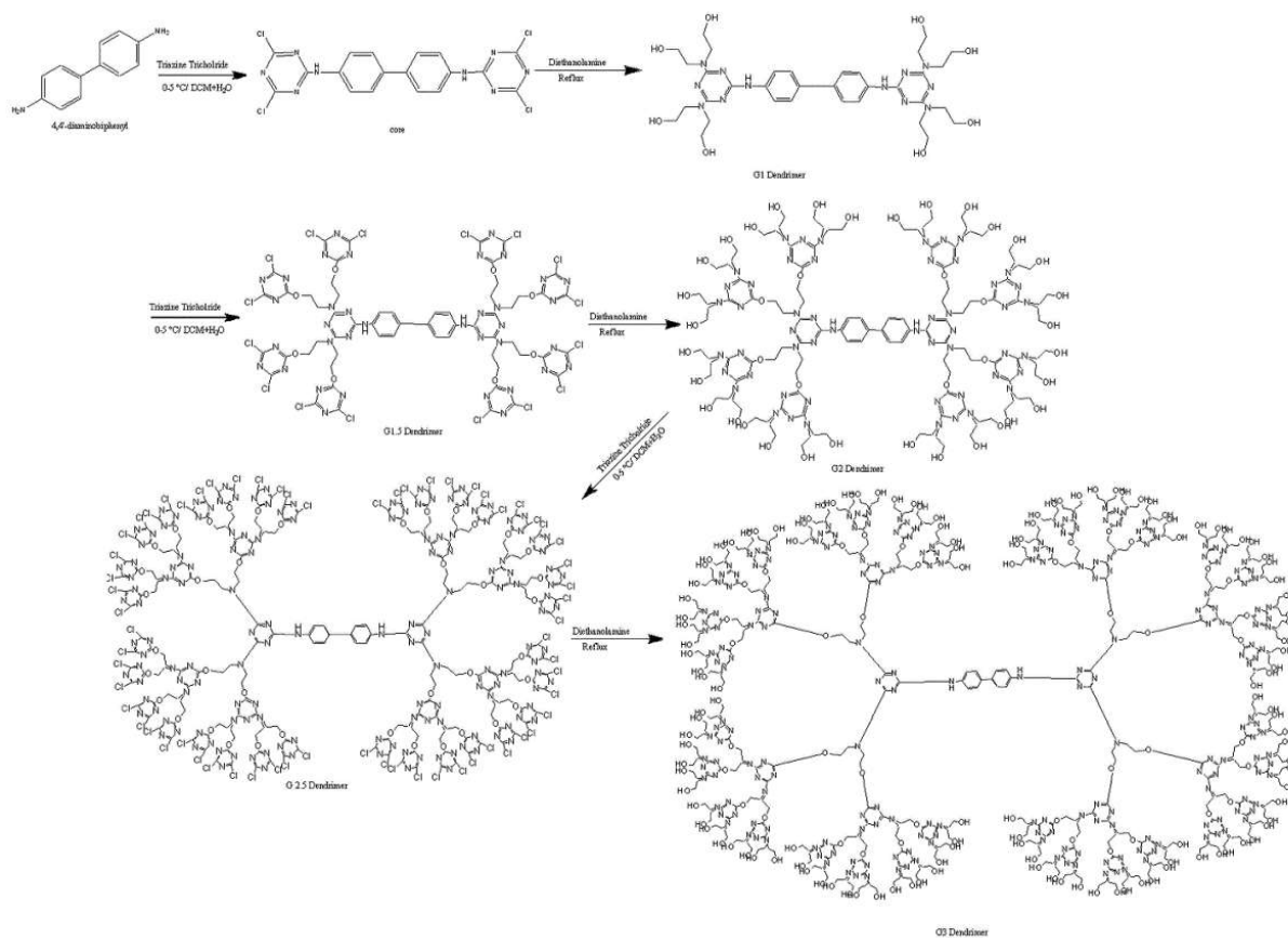
Figure 1 Synthesis of Generation 3 Triazine based Dendrimer
