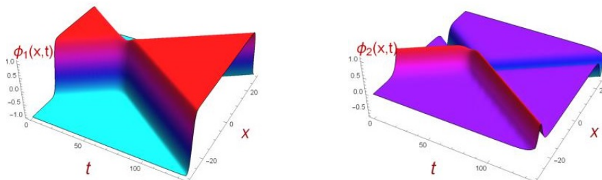
Figure 16: Evolution of the first (left) and second component (right) in the K^{(q,\lambda)} - K^{(-q,-\lambda)} collision with impact velocity v_0 = 0.3 for the model parameter \sigma = 0.72 . The kink K^{(q,\lambda)}(v_0) and the antikink K^{(-q,-\lambda)}(-v_0) (of different type) collide and elastically reflect ( elastic reflection regime ).
