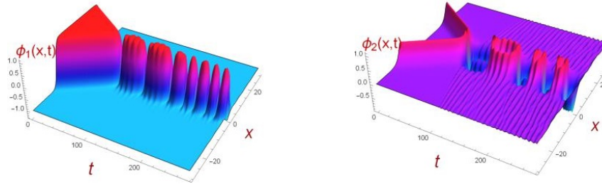
Figure 12: Evolution of the first (left) and second component (right) in the K^{(q,\lambda)} - K^{(-q,\lambda)} collision with impact velocity v_0 = 0.15 for the model parameter \sigma = 0.72 . The kink and its own antikink collide and form a bound state where a transmutation occurs after every kink collision ( bion formation regime ).
