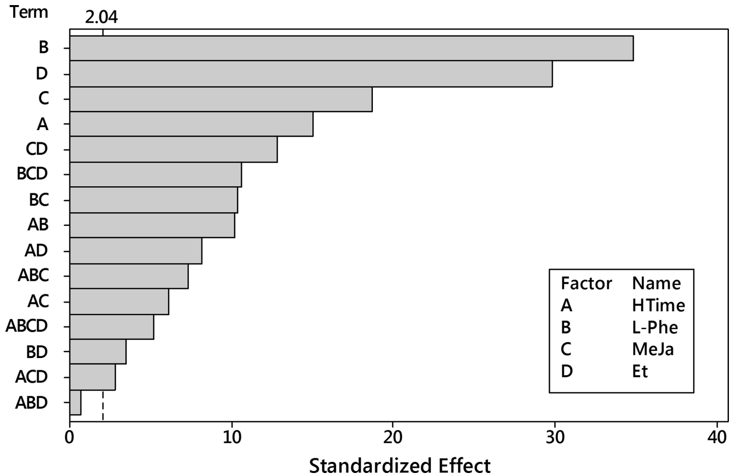
Fig 15. Pareto plot of standardized effects for the transformed harpagide outcome. Four factors (HTime, L-Phe, MeJa, Eth) and their interaction up to the 4 th order were considered. Significance level \alpha = 0.05 , t = 2.042 .
