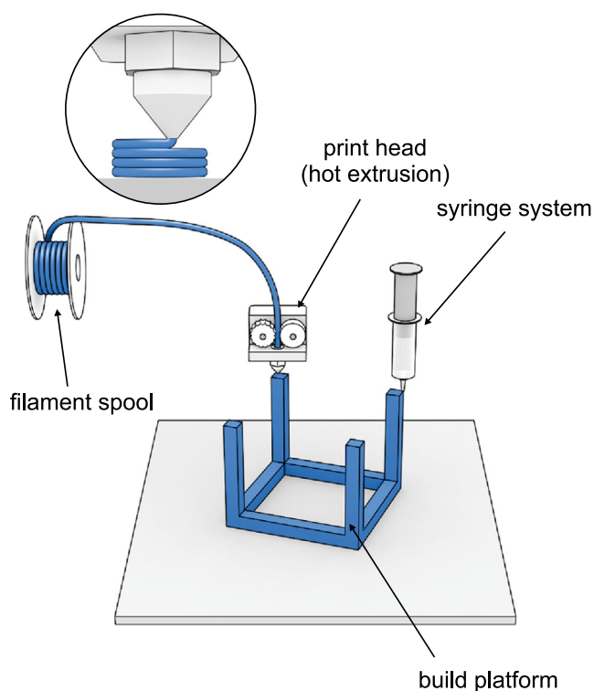
Fig. 10 Extrusion-based techniques.
