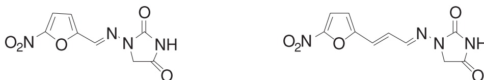
Figure 1. Chemical structure of nitrofurantoin (E)-1-[(5-nitro-2-furyl)methylideneamino]imidazolidine-2,4-dione and furazidin (1-[3-(5-nitro-2-furyl)prop-2-en-1-ylidene]amino]imidazolidine-2,4-dione)
