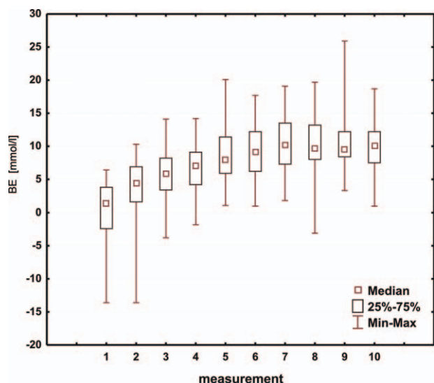
Figure 5. Box and whisker plot for values of BE. BE = base excess.
