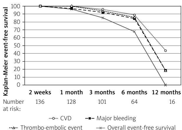
Figure 3. Kaplan-Meier curves showing event-free survival of patients on active triple therapy (TT). No patients with TT lasting 12 months were free from complications
