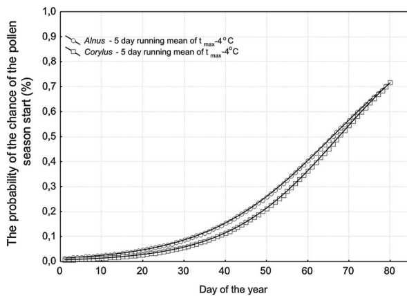
Fig. 4 The graphs of logistic regression function presenting the probability of the pollen season occurrence for Alnus and Corylus at two threshold temperatures ( -4 and 4^{\circ}\text{C} ) in
