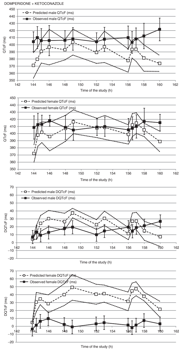
Figure 4 Observed (black squares) and predicted (empty squares) QTc and DQTcF values for domperidone plus ketoconazole therapy (±SD) in domperidone with ketoconazole scenario.
