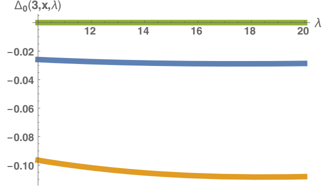
FIG. 12. Binding energy (78) vs \lambda for m_H \rightarrow \infty : x = \frac{1}{3} green (upper) curve, x = \frac{2}{3} lower (orange) curve, and x = \frac{3}{3} middle (blue) curve.
