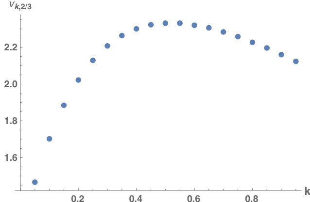
FIG. 11. \nu_{k,2/3} vs k for x = \frac{2}{3} and m_H \rightarrow \infty .
