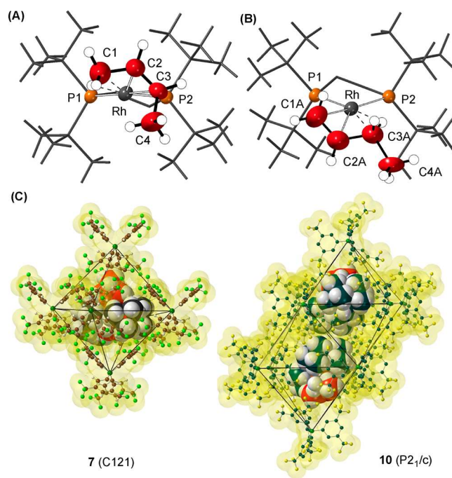
Figure 2. Solid-state structures of the cation 10 (A) and 11 (B). [\text{BAR}^F_4]^- anions and most hydrogen atoms omitted. Displacement ellipsoids shown at the 50% probability level. Selected bond lengths (Å), 10: Rh–C2, 2.168(6); Rh–C3, 2.356(9); Rh–C1, 2.418(9); C1–C2, 1.474(13); C2–C3, 1.347(13); C3–C4, 1.347(13). 11: Rh–C1A, 2.250(8); Rh–C2A, 2.154(6); Rh–C3A, 2.349(9); C1A–C2A, 1.363(14); C2A–C3A, 1.525(14); C3A–C4A, 1.363(14). (C) Packing diagram of 7 and 10 showing the arrangement of [\text{BAR}^F_4]^- anions. Cations and isosurface shown at van der Waals radii.
