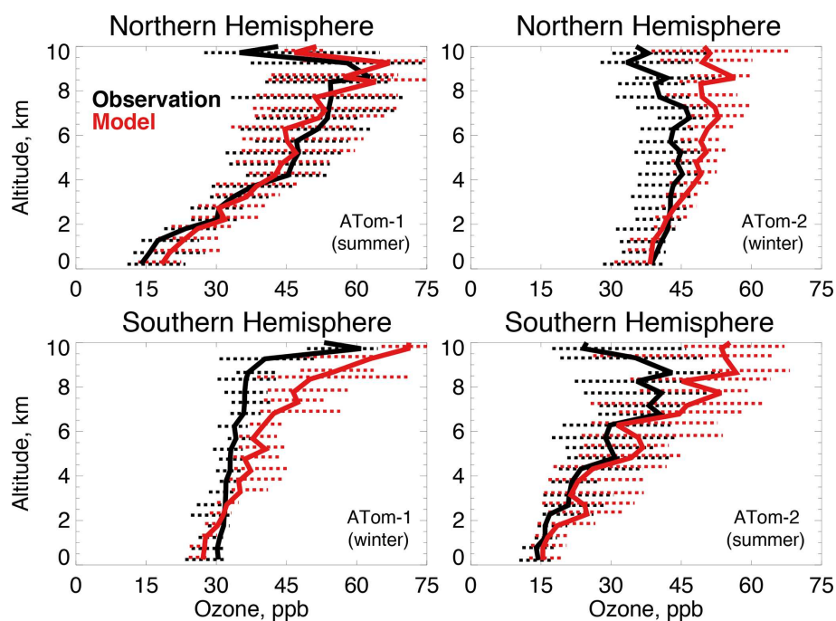
Figure 6. The same as Fig. 3 for median ozone concentrations. Ozone was measured by the NOAA NO_yO_3 instrument as described in Table 2.
