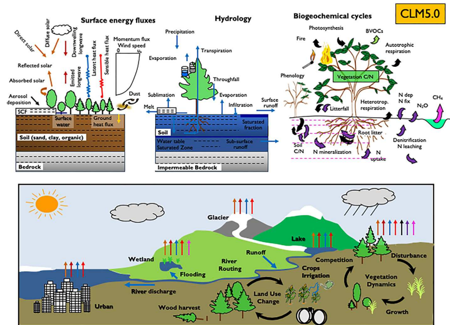
Figure 1. Schematic representation of primary processes and functionality in CLM5. SCF = snow cover fraction; BVOC = biogenic volatile organic compounds; C/N = carbon and nitrogen. For biogeochemical cycles, black arrow denotes carbon flux, and purple arrow denotes nitrogen flux. Note that not all soil levels are shown. Not all processes are depicted. Optional features that are not active in default configurations are italicized. Updated from figure 1 in Lawrence et al. (2011).
