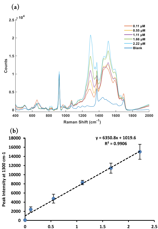
Figure 5. (a) SERS spectra obtained upon addition of various concentrations of TNT to 3-mercapto-2-butanone anion and subsequent addition to silver nanoparticles. All spectra were collected using a Renishaw Plate Reader with a 532 nm excitation wavelength (100 mW) and a 0.8 s acquisition time. (b) Plot of the intensity of the 1300 \text{ cm}^{-1} peak against TNT concentration ( \mu\text{M} ) showing a linear relationship in the range 0.1–2.2 \mu\text{M} (coefficient of determination R = 0.99 ). Error bars indicate the standard deviation on 3 replicate samples with 5 measurements taken of each.
