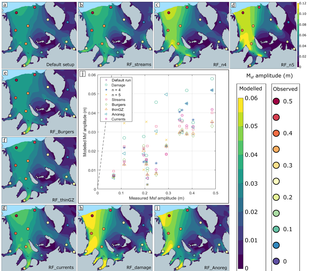
Figure 4. M_{sf} amplitude on the Ronne Ice Shelf for nine of the model experiments (a–i) outlined in Table 1. Note the different colour scale used for experiment “RF_n5” in panel (d). Observed M_{sf} amplitudes from GPS observations are indicated in panel (a) by coloured circles. Panel (j) compares measured and modelled M_{sf} amplitude at each of the marked locations for the same set of experiments. Note that in producing this figure we use an evenly distributed subset of measurements to avoid bias in areas with more measurements and thus make interpretation of the overall misfit across the entire ice shelf easier.
