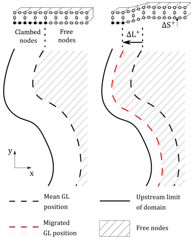
Figure E1. Plan view of a grounding zone, showing how grounding line motion is imposed in the model. Initially the model runs with no tides until it has visco-elastically relaxed. Nodes upstream of the grounding line are clamped at the base and nodes downstream have no constraints. Once tides are switched on, the grounding line can migrate upstream ( \Delta L^+ ) or downstream ( \Delta L^- ) and nodes that are outside of the defined grounded area have any constraints removed.
