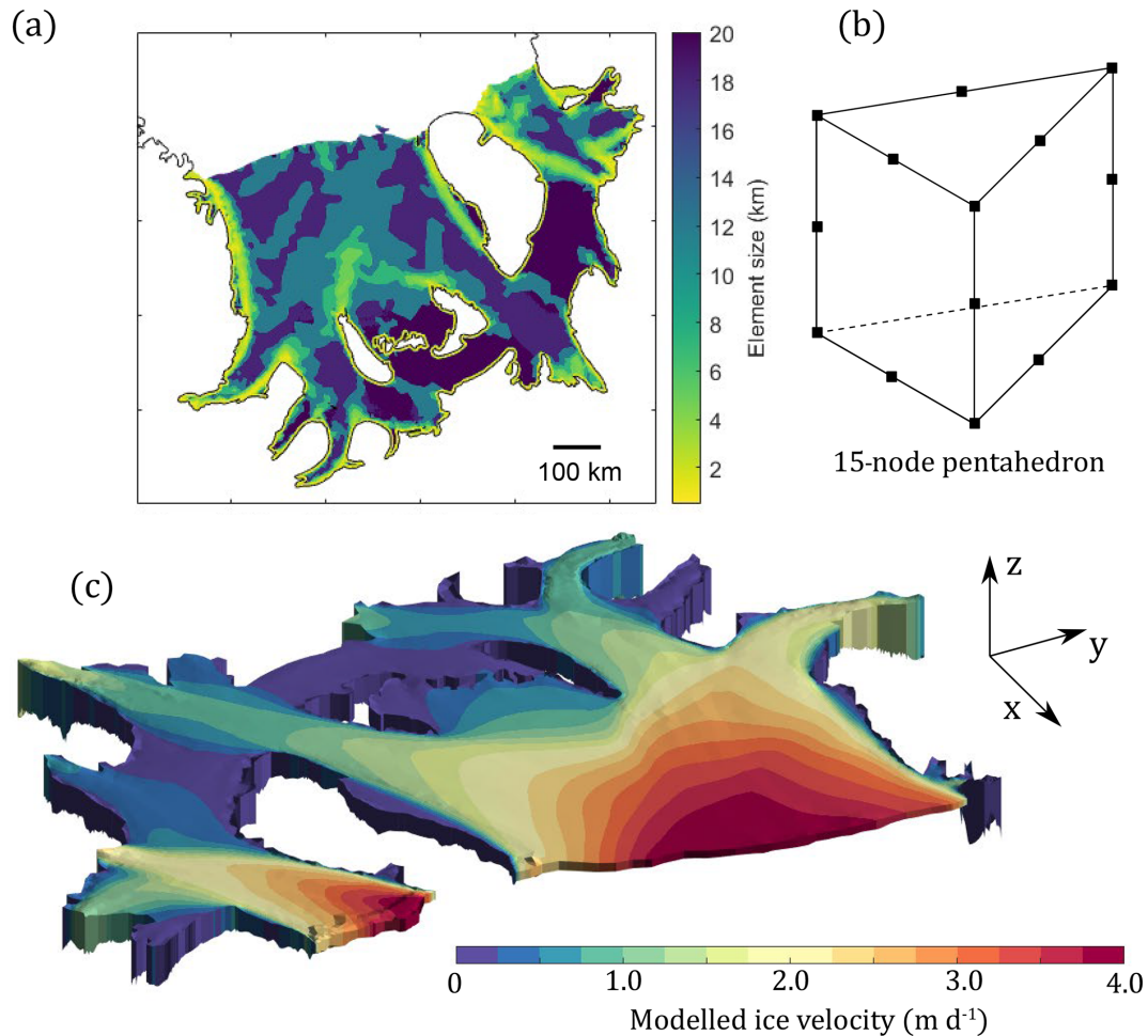
Figure 2. Overview of the finite-element model, showing model resolution (a), the quadratic pentahedral elements used (b) and a vertically exaggerated oblique view of the model showing modelled mean ice velocity for the default setup experiment (c).
