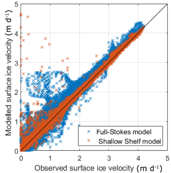
Figure A1. Comparison between observed surface ice velocities, obtained from the MEaSURES version 2 dataset (Rignot et al., 2017, 2011b; Mouginot et al., 2012), and modelled ice velocities using either the 3-D model (Sect. 2.1, blue crosses) or the \dot{U}a model (red crosses).
