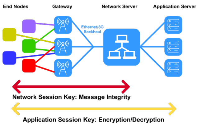
Fig. 1: Example LoRaWAN session.
