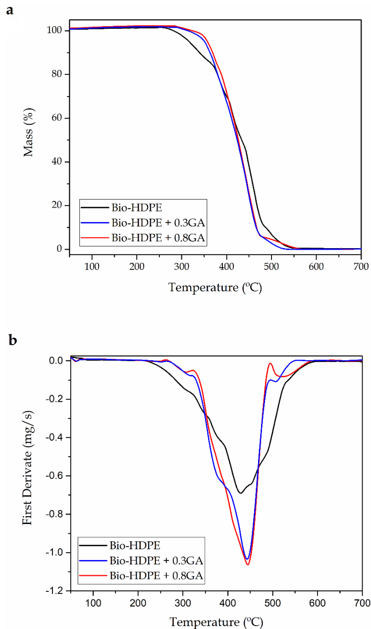
Figure 4. (a) Thermogravimetric analysis (TGA) curves and (b) first derivative (DTG) of the bio-based high-density polyethylenes (bio-HDPE) films containing different amounts of gallic acid (GA).
