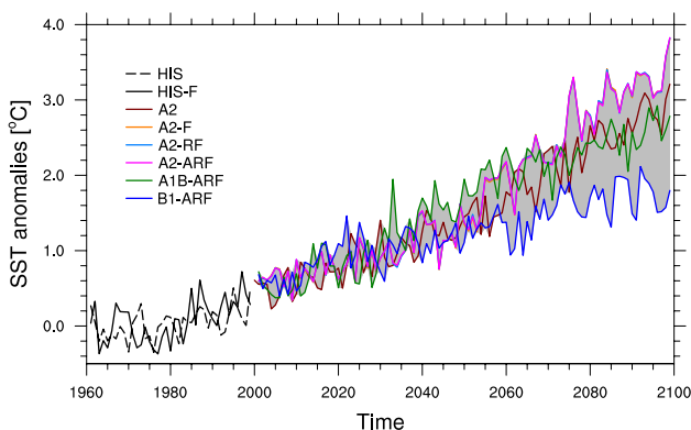
Fig. 12 Yearly mean time series of sea surface temperature anomalies (vs. 1961–1990) averaged over the Mediterranean basin. A2-F, A2-RF and A2-ARF curves are overlapping. The spread of the ensemble is shaded in grey
