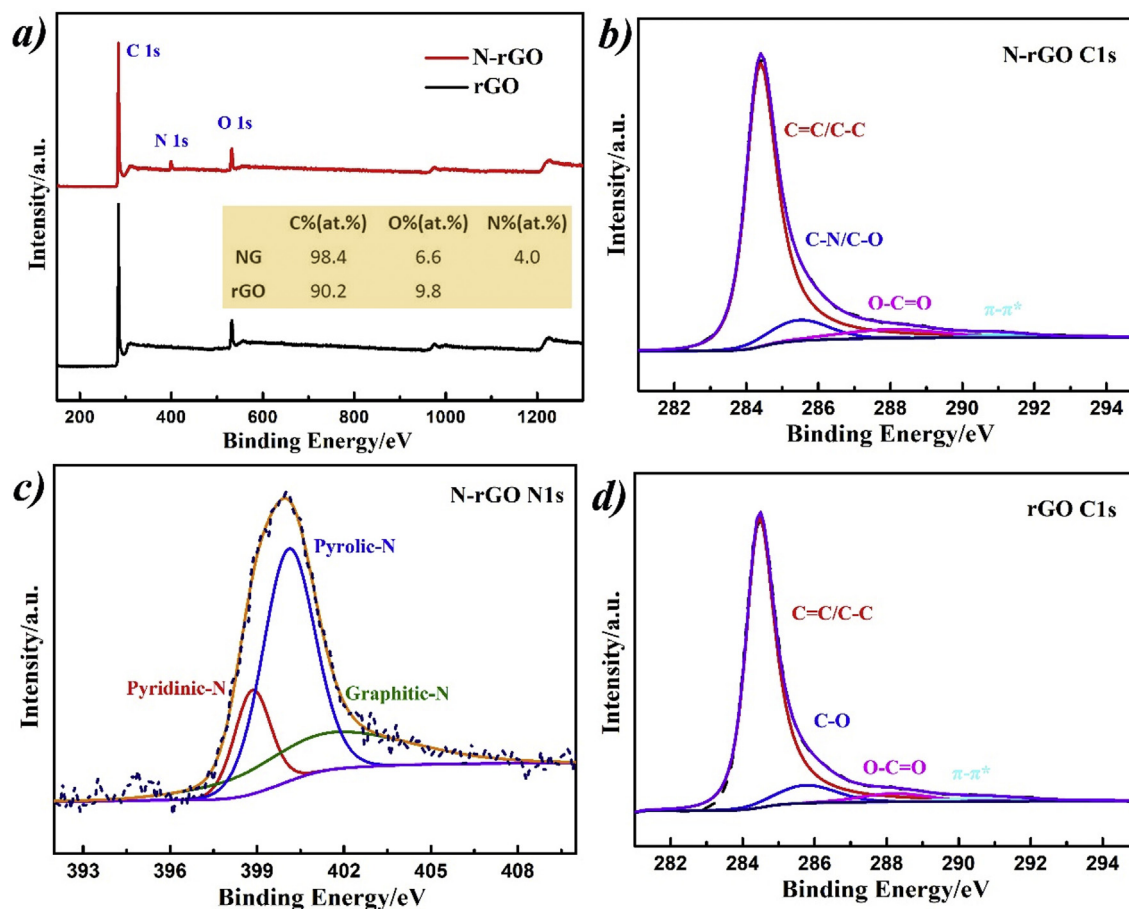
Fig. 1. XPS data for N-rGO and rGO. (a) XPS survey scan spectra of N-rGO and rGO, the inset table shows the elemental content of each sample; (b) C 1s and (c) N 1s spectra of N-rGO; (d) C 1s spectra of rGO. (A colour version of this figure can be viewed online.)
