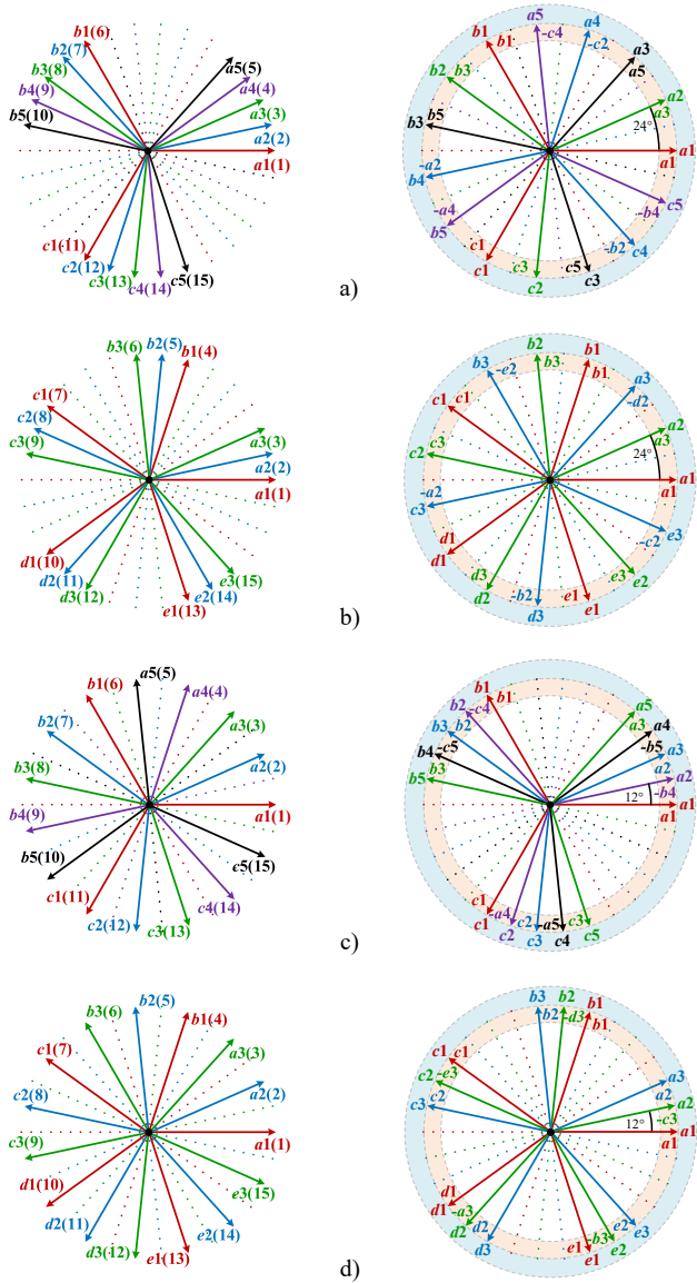
FIGURE 6. Winding reconfiguration in fifteen-phase machine.
