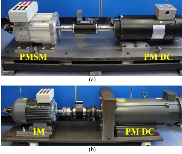
FIGURE 9. Nine-phase PMSM (a) and induction machine (b) experimental setups.
