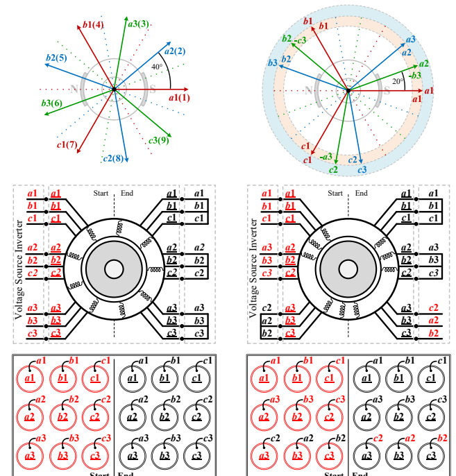
FIGURE 5. Symmetrical to asymmetrical winding reconfiguration: magnetic axis diagram (upper), VSI power supply leads rearrangement at the machine's terminal box (middle), and old and new mimic diagrams (bottom plots).
