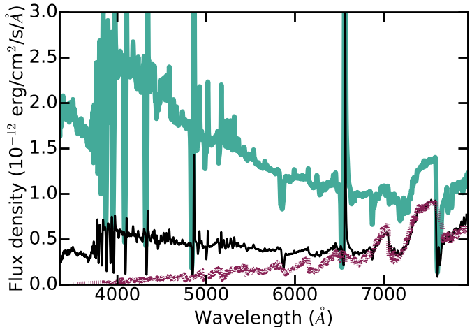
Figure G1. Optical spectra of MWC 560 used to calculate luminosities: the brightest outflow fast state spectrum (2016 Apr 3), a quiescent state spectrum (2015 Mar 10) typical for the present decade, and the Case M5 giant template from Fluks et al. (1994) scaled by eye to match the red side of the quiescent spectrum (which leads to the smoothest residuals). The MWC 560 spectra are corrected for extinction with E(B-V)=0.15 (Appendix A). The differing spectral slopes are primarily due to the additive contribution of the giant, which has a smaller fractional contribution during the outflow fast state. Only low-resolution spectra are plotted here, decreasing the prominence of narrow metal emission lines.
