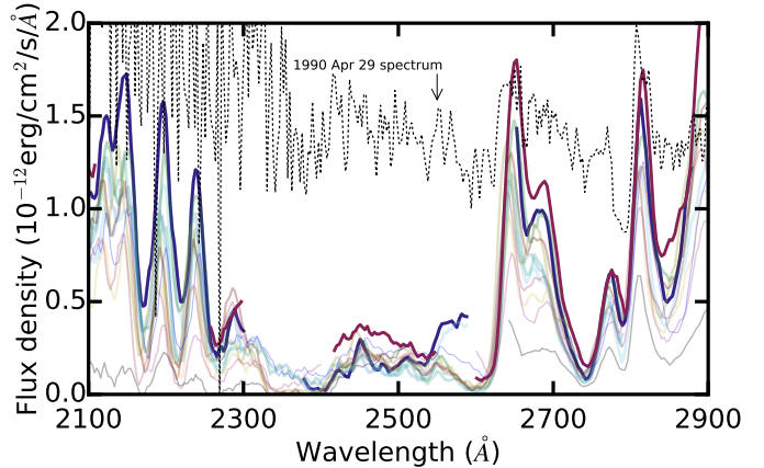
Figure 5. The Swift UV spectra (obtained between 2016 March and June; all solid lines) demonstrate substantial variability in normalization but not in shape, and signify a persistent iron curtain absorbing on a varying continuum throughout the 2016 observations. In particular, the varying flux near 2650 Å and at the \text{Mg II } \lambda 2800 \text{ \AA} emission line suggest that the varying normalization cannot be attributed to varying opacity. The 1990 April 29 spectrum (dashed black line) is included for comparison, and approximates the underlying continuum at the NUV flux maxima of 2016 March 2 (dark blue line) and 2016 April 4 (dark red line). Omitted from this plot are all regions in individual spectra where image inspection suggested zeroth-order contamination, as well as the three spectra noted in Table B1 as having nearby bright first order flux or suffering from underestimated flux due to loss of lock. All spectra were de-reddened by E(B-V)=0.15 ( Schmid et al. 2001 , and our Appendix A ).
