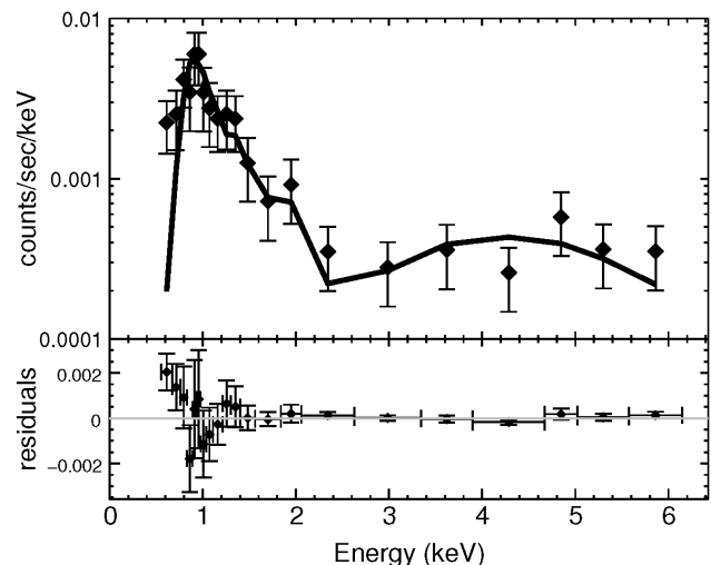
Figure 3. The background-subtracted X-ray spectrum obtained with Chandra on 2016 March 8–9, displayed with grouping to bins of at least 10 counts and fit with the 2-component soft+hard fit described in the text and Table 3. The fit itself was performed on the spectrum grouped to bins of at least 20 counts. The vertical axis is logarithmic for the spectrum and linear for the residuals.
