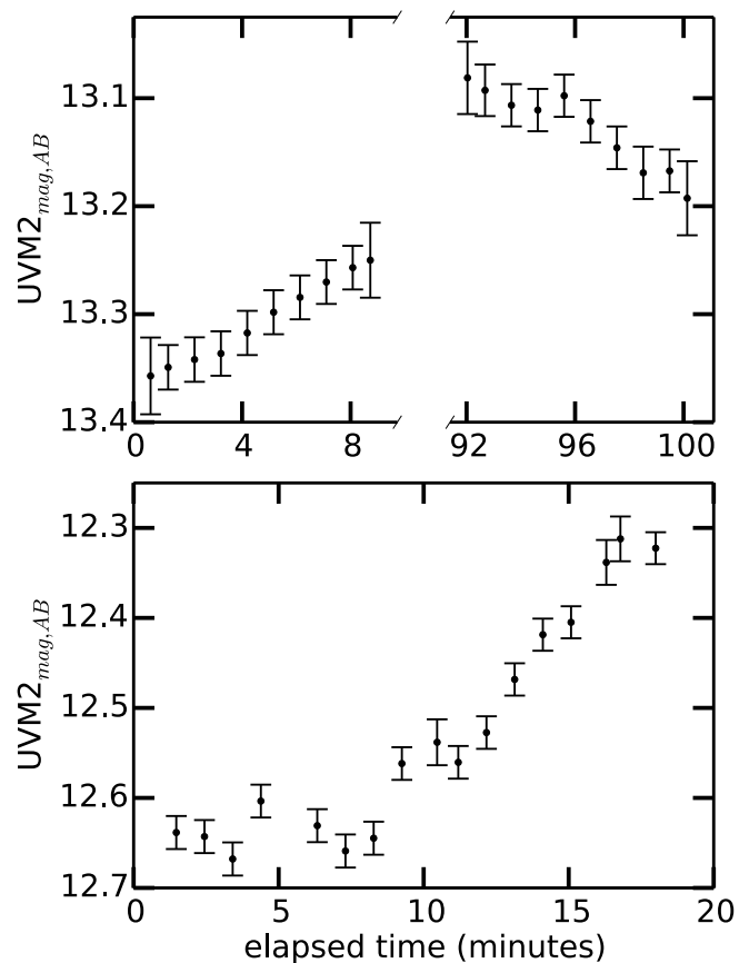
Figure 7. Example light curves from our Swift UVOT observations. These changes in NUV flux, up to 40% on a time-scale of minutes, are consistent with flickering from the accretion disc. Swift UVM2 AB magnitude is plotted against minutes since 2016 June 1 at about 18:23 UTC (MJD= 57540.7661081, top panel, with a break in the time axis during which observations were interrupted) and 2016 March 5 at about 5:39 UTC (MJD= 57452.235247, bottom panel).
